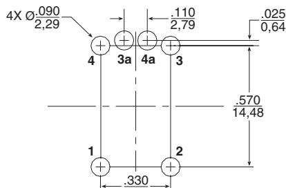
SUGGESTED PAD LAYOUT - (PA0032/33)
