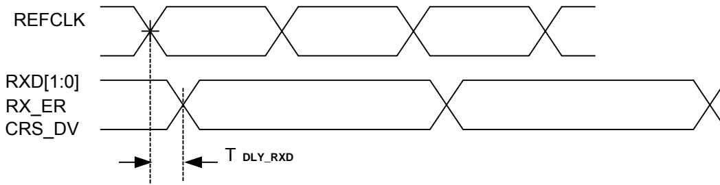
Figure 5: Receive Delay
