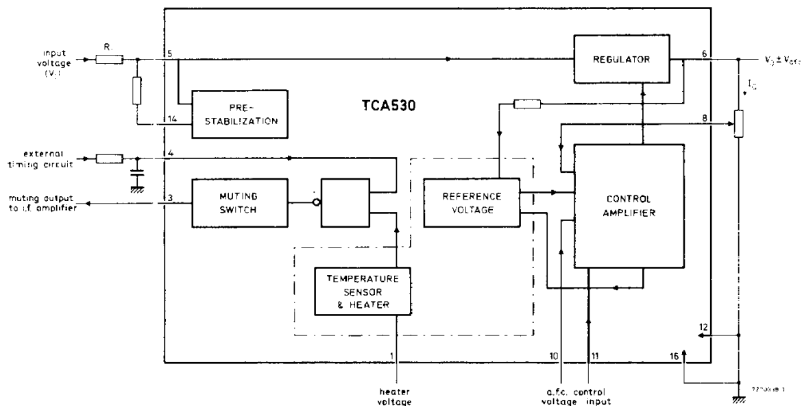
Fig. 1 Block diagram.
