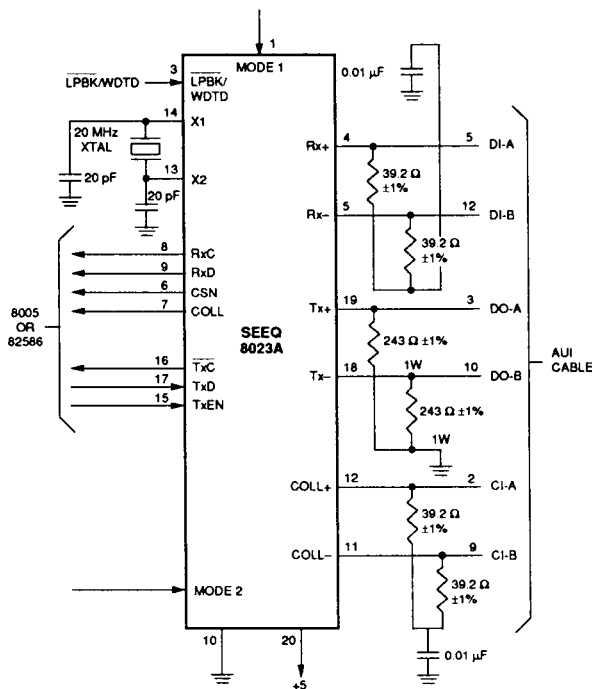
Figure 4. 8023A Interface
