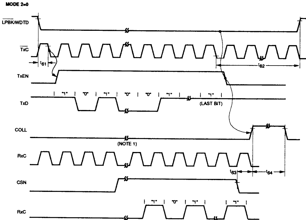
Figure 13. Loopback Timing
