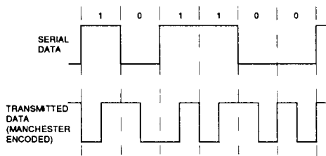
Figure 2. Manchester Coding
