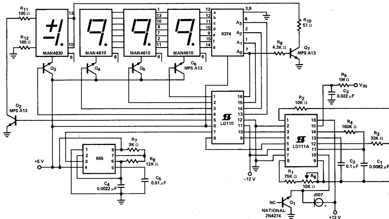
3 1/2 Digit DVM ( \pm 200.0 mV) Common Anode Display
