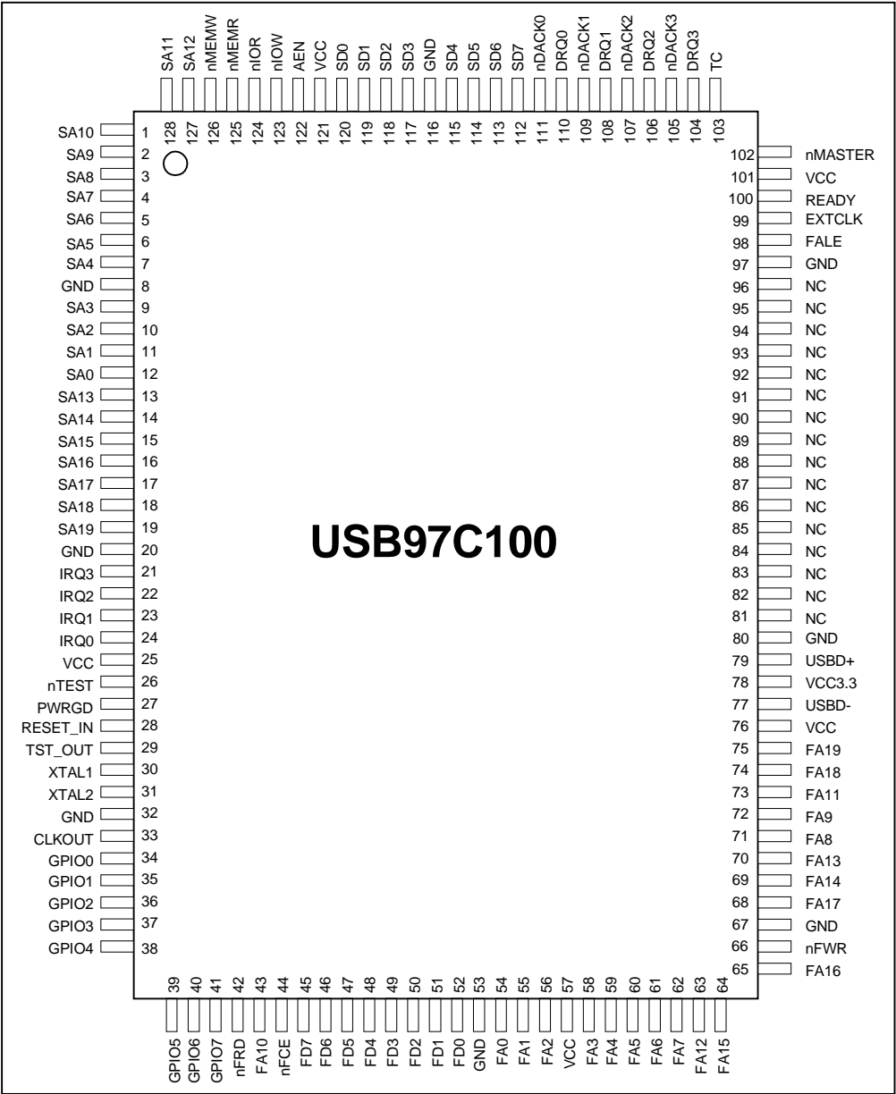
FIGURE 1 - PIN CONFIGURATION
