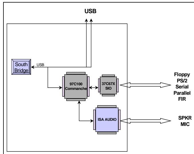
TYPICAL PC MOTHERBOARD APPLICATION
