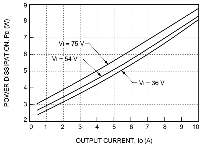
Figure 27. JW050F Power Dissipation vs. Output Current
