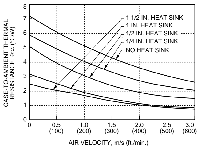
Figure 32. Case-to-Ambient Thermal Resistance Curves; Either Orientation
