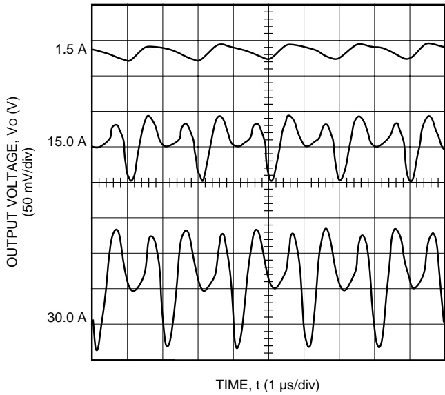
Figure 13. Typical JW150F Output Ripple Voltage at Room Temperature, I_o = \text{Full Load}
