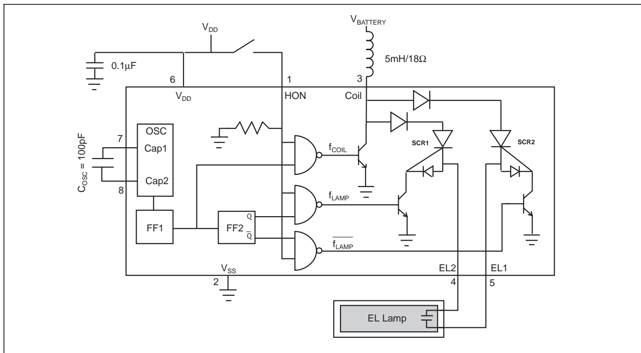
SP4422A Schematic
