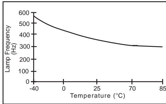
Lamp Frequency vs. Temperature V_{DD}=3.0V ; Coil=5mH/18 \Omega ; C_{OSC}=100pF ; Load=10nF
