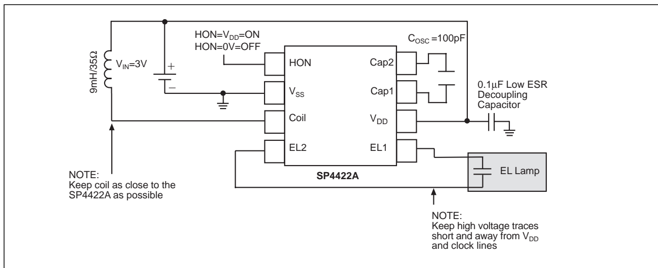
Typical SP4422A Application Circuit
