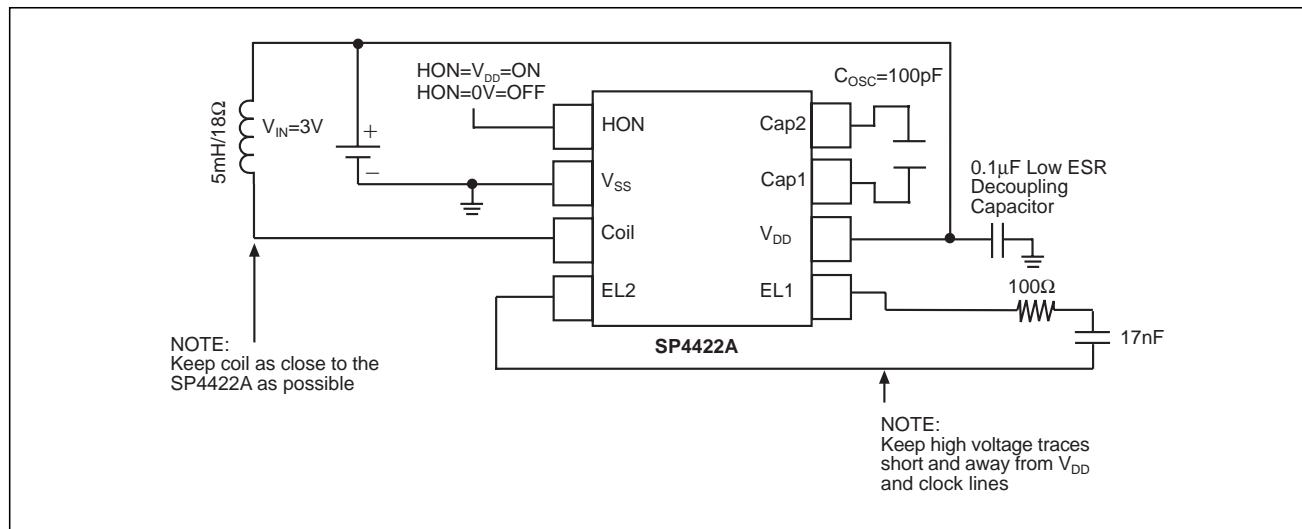
SP4422A Test Circuit
