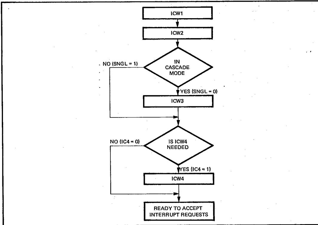
Figure 4. Initialization Sequence
