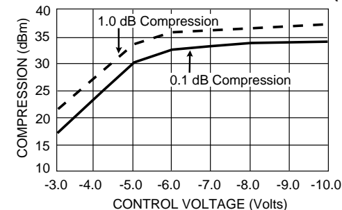
COMPRESSION vs CONTROL VOLTAGE (900 MHz)
