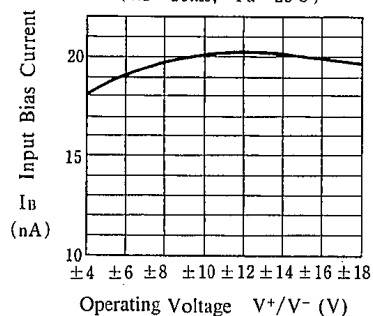
Input Bias Current vs. Operating Voltage
