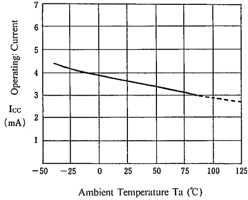
Operating Current vs. Temperature ( V^+/V^- = \pm 15V )
