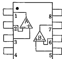
NJM1458D NJM1458M
