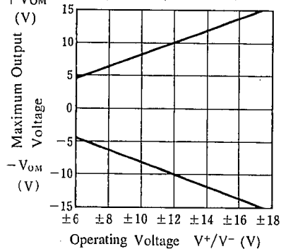
Maximum Output Voltage Swing vs. Operating Voltage
