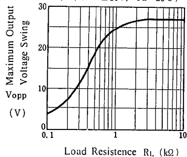
Maximum Output Voltage Swing vs. Load Resistance
