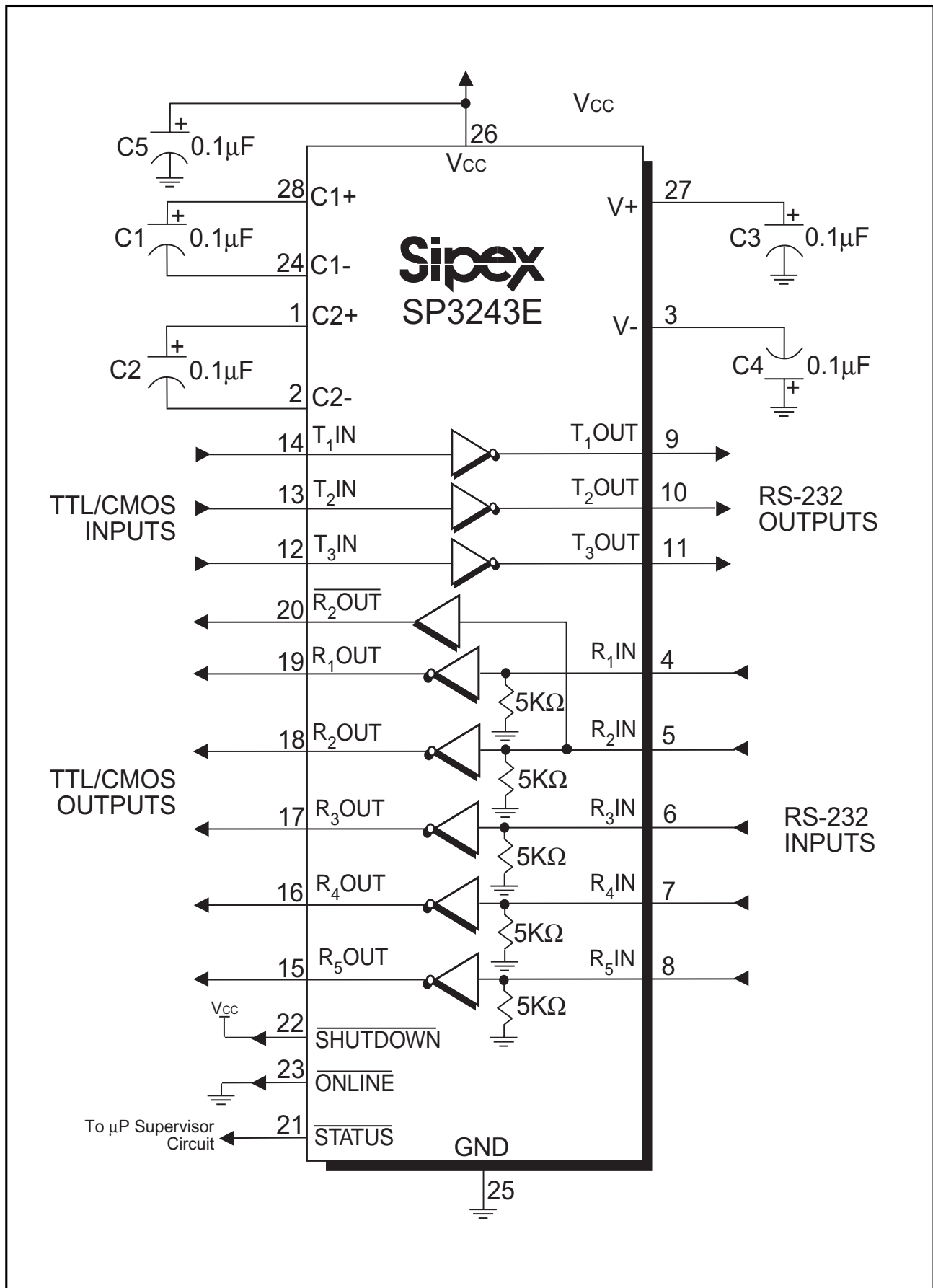
Figure 10. SP3243E Typical Operating Circuit
