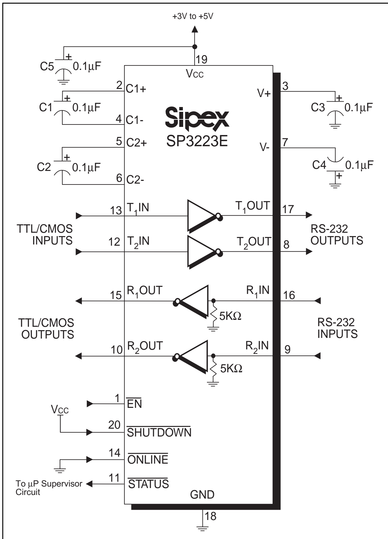
Figure 9. SP3223E Typical Operating Circuit
