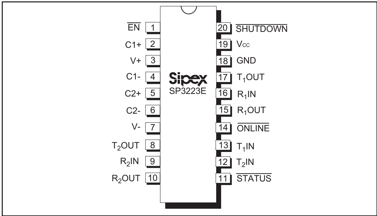
Figure 7. SP3223E Pinout Configuration
