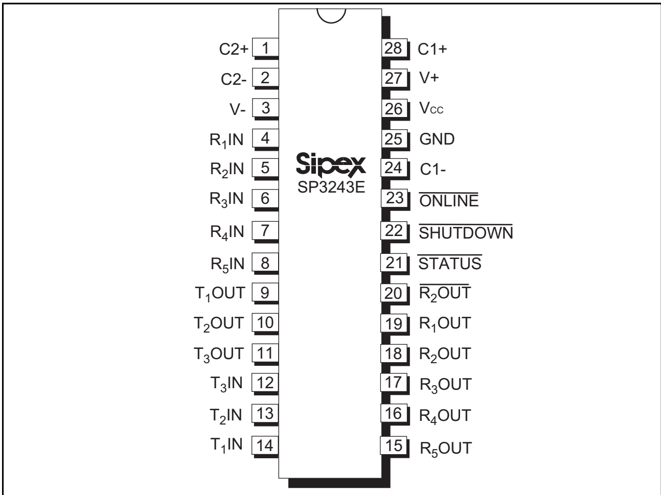
Figure 8. SP3243E Pinout Configuration
