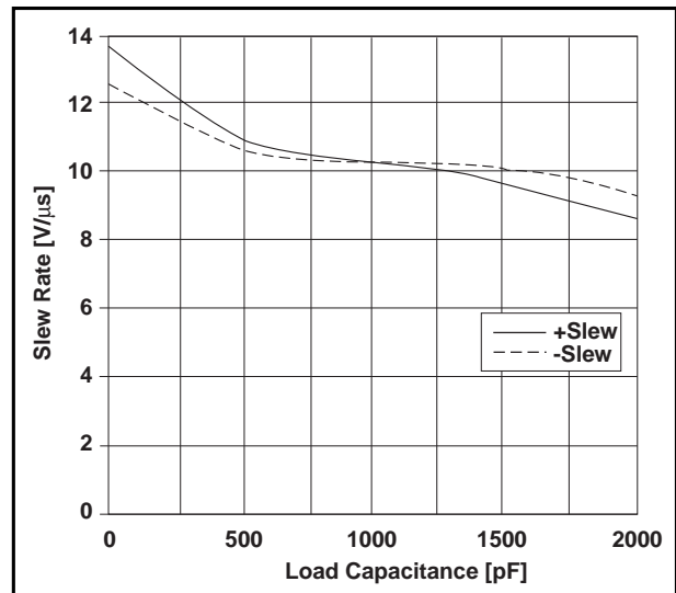
Figure 2. Slew Rate VS. Load Capacitance for the SP3223E
