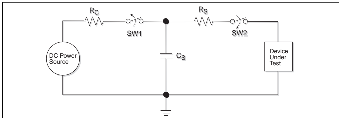
Figure 25. ESD Test Circuit for Human Body Model
