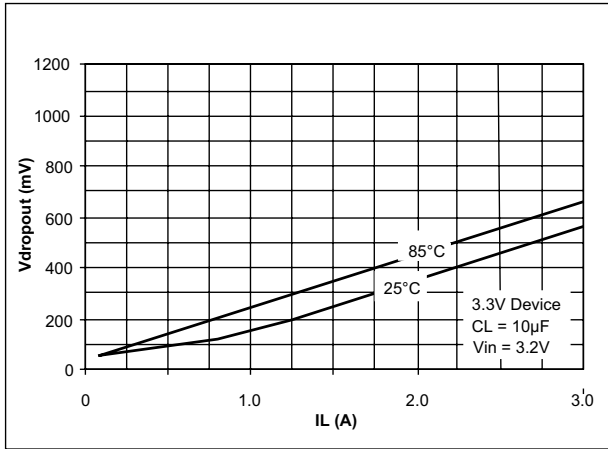
Figure 3. Dropout Voltage vs Load Current
