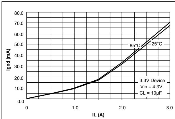
Figure 5. Ground Current vs Load Current
