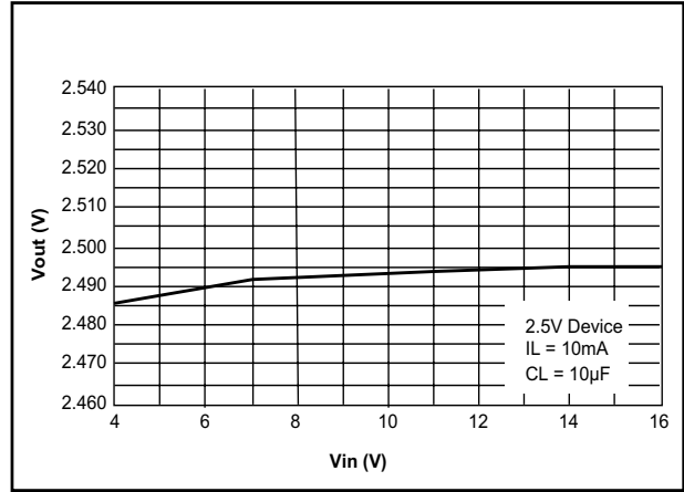
Figure 4. Line Regulation
