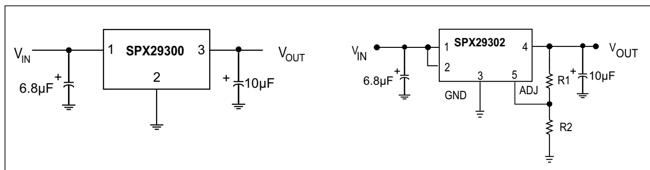
Figure 1. Fixed Output Linear Regulator
