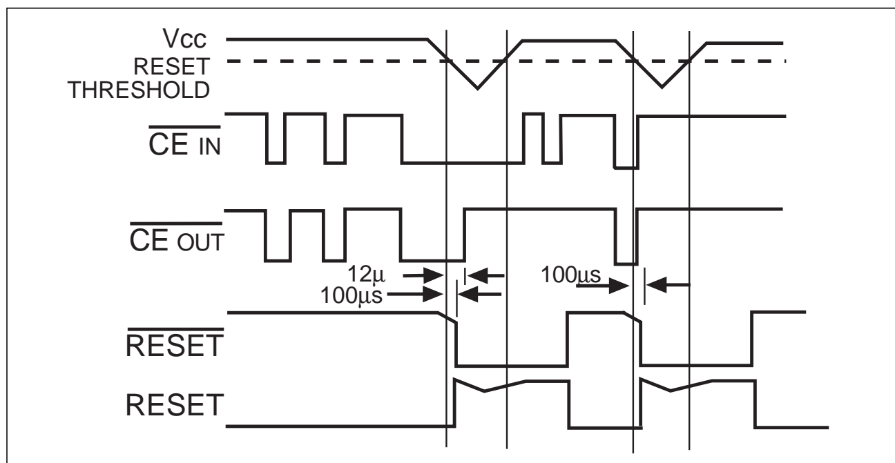
Figure 19. Reset and Chip-Enable Timing
