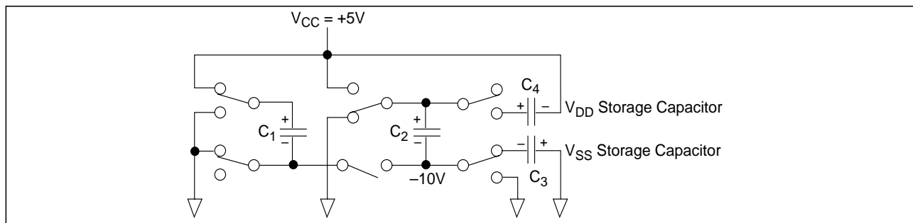
Figure 5. Charge Pump — Phase 2
