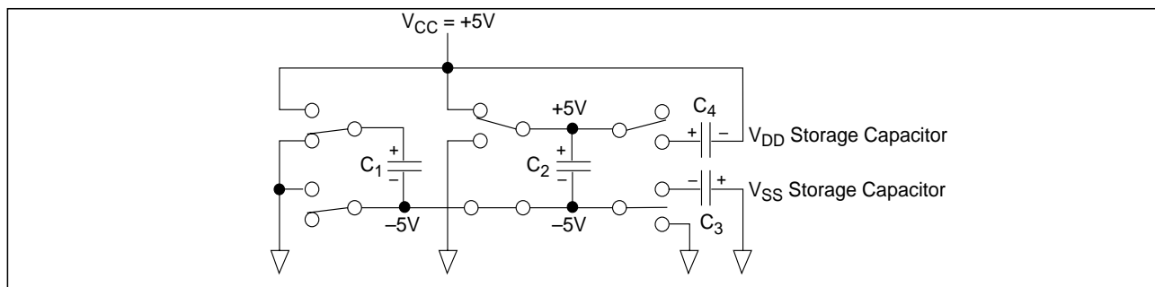
Figure 4. Charge Pump — Phase 1
