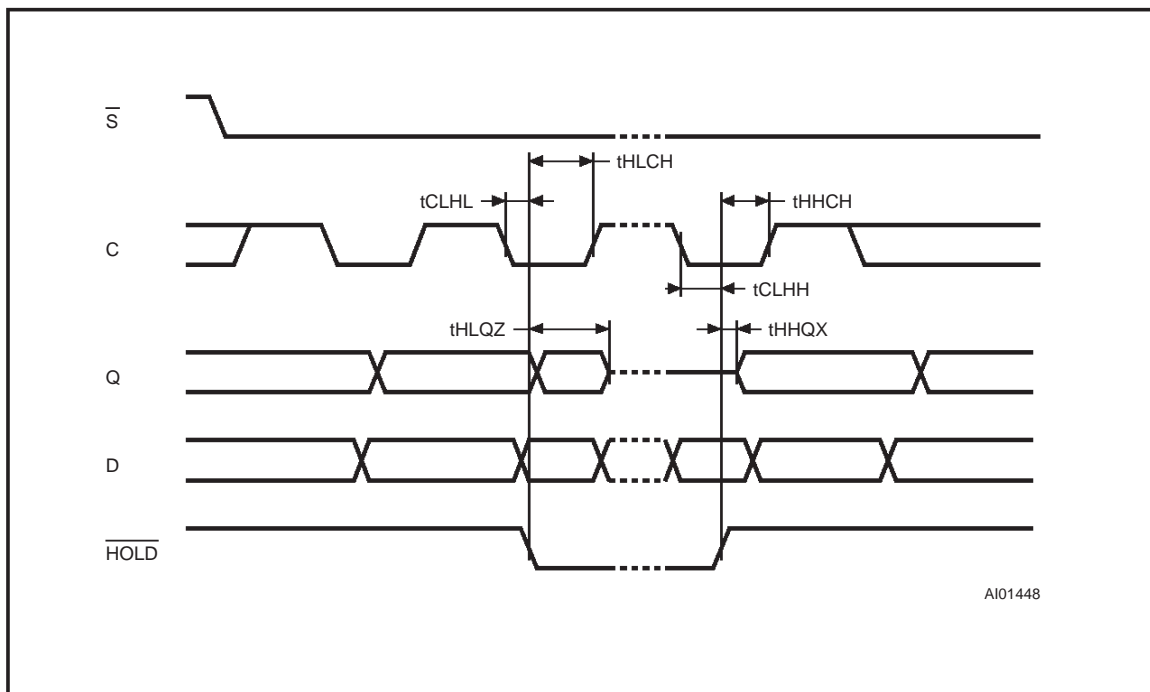
Figure 15. Hold Timing
