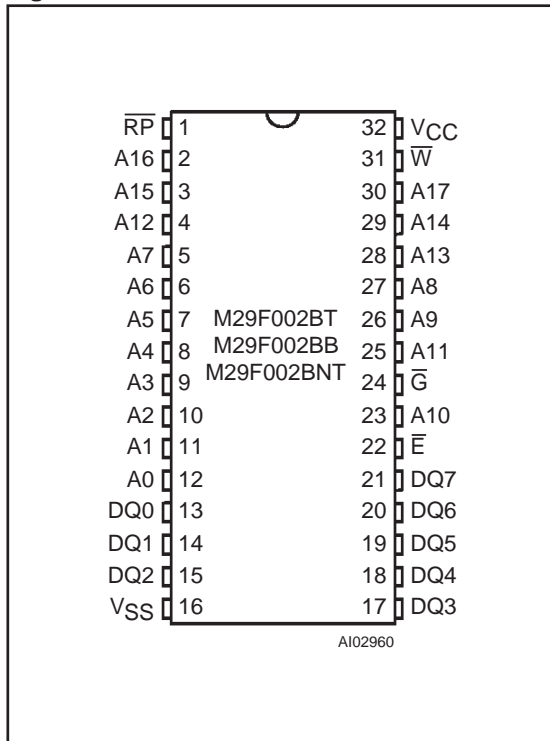
Figure 2C. PDIP Connections
