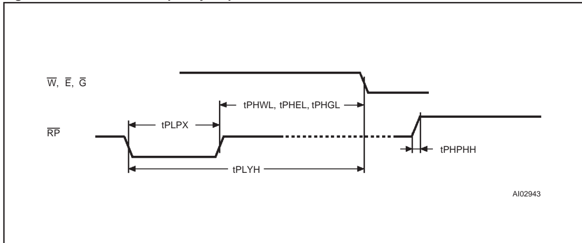
Figure 10. Reset/Block Temporary Unprotect AC Waveforms
