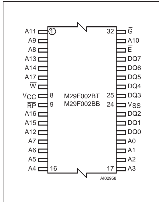
Figure 2B. TSOP Connections
