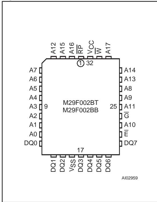
Figure 2A. PLCC Connections
