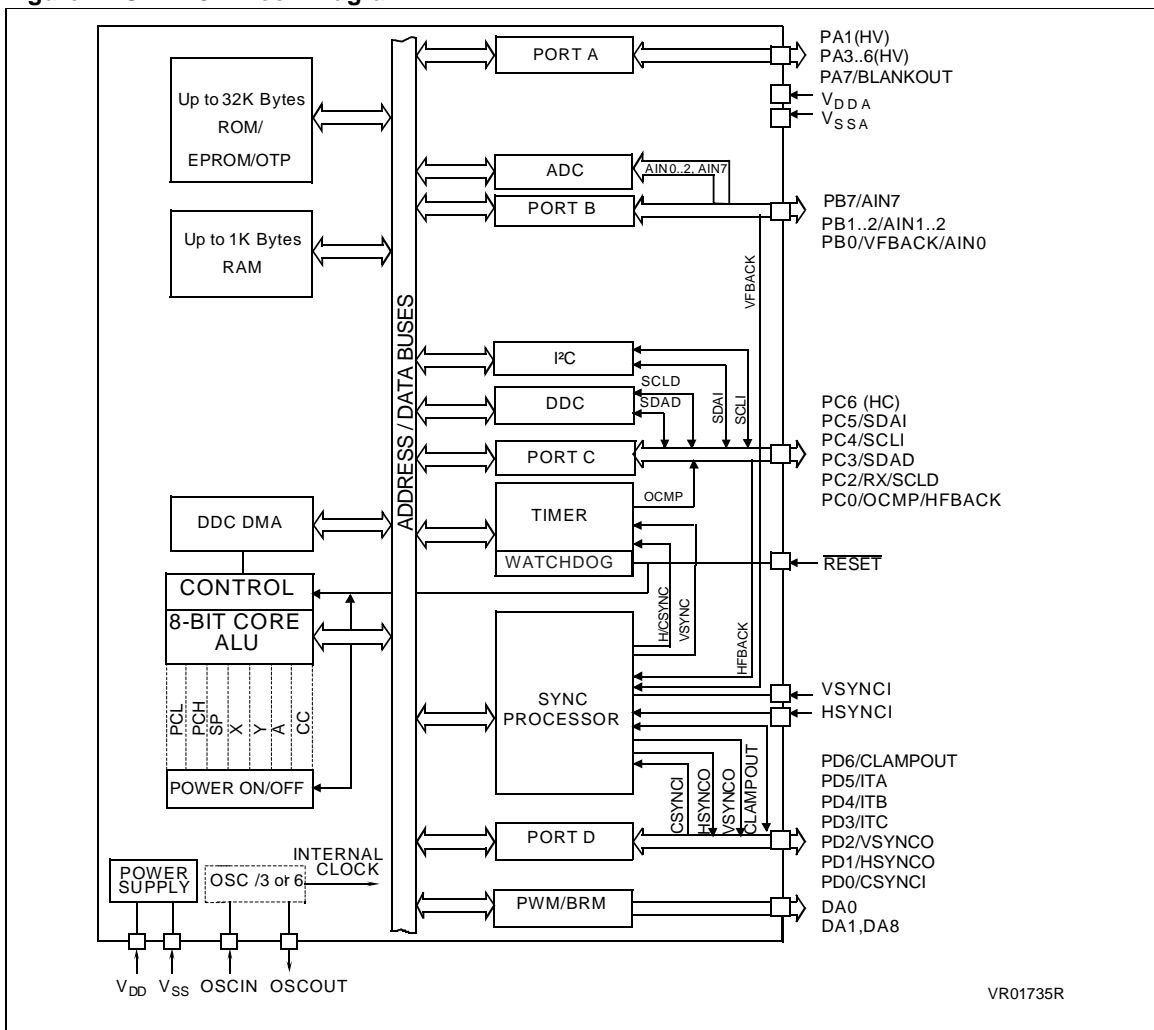
Figure 1. .ST72752 Block Diagram
