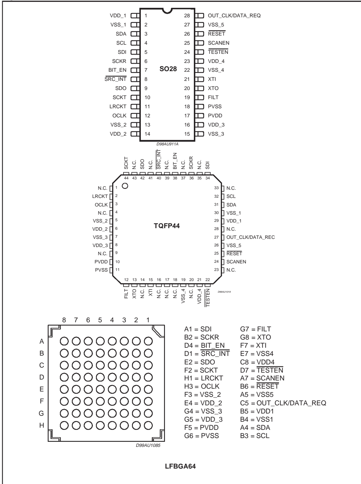
Figure 2. Pin Connection
