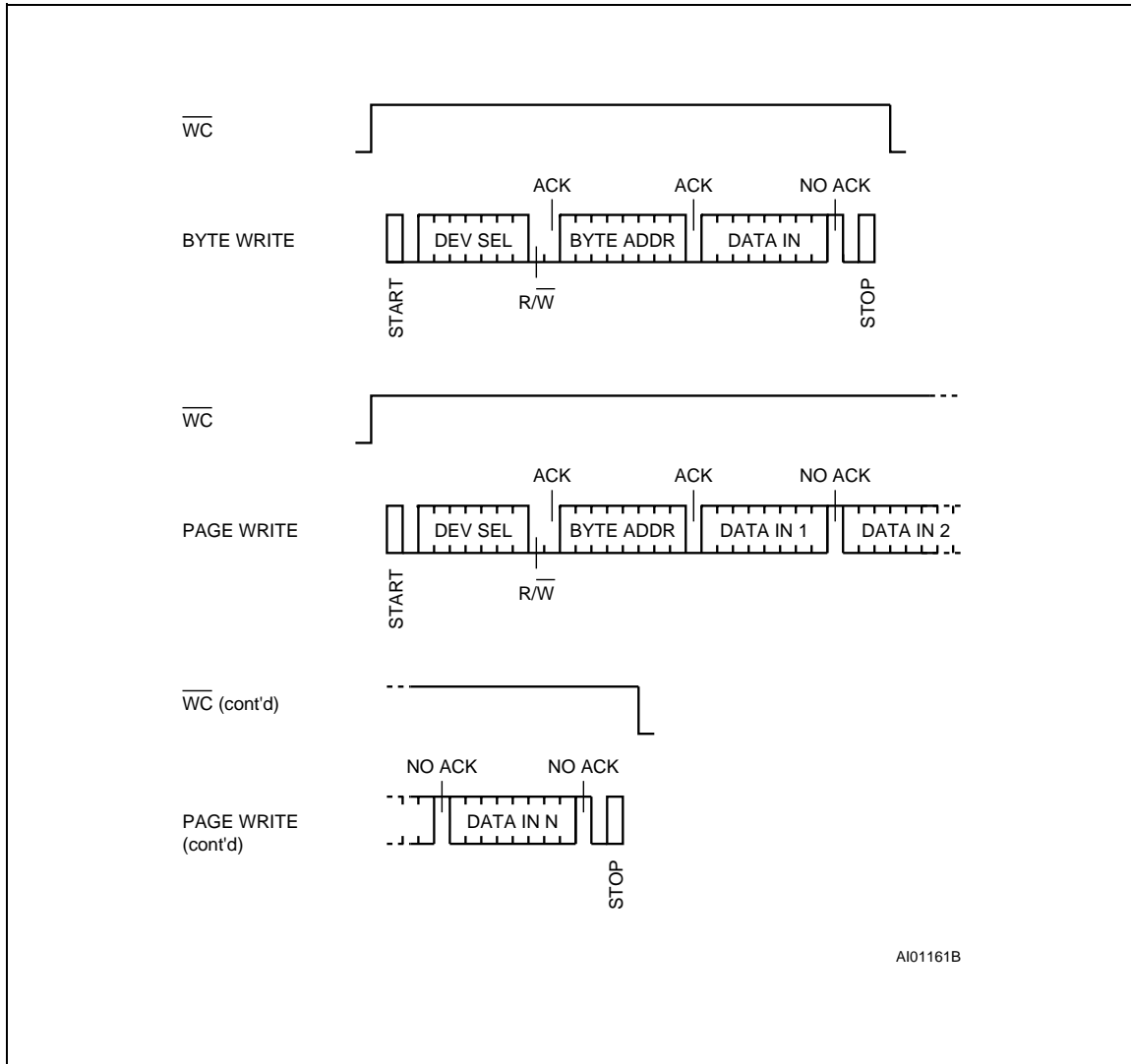
Figure 9. Write Modes Sequence with Write Control = 1 (ST24/25W01)
