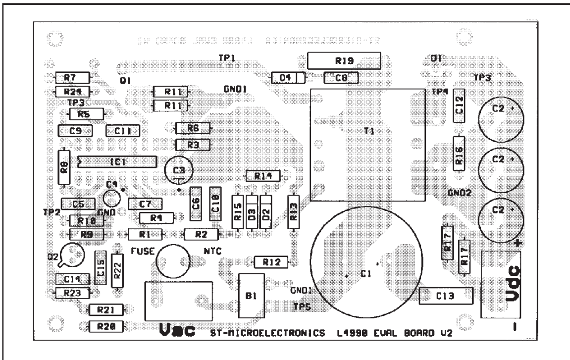
Figure 32. AC-DC adaptor PCB layout (1.25 :1 scale) - Back Side.
