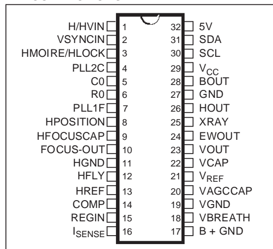
SHRINK32 (Plastic Package) ORDER CODE: TDA9111
