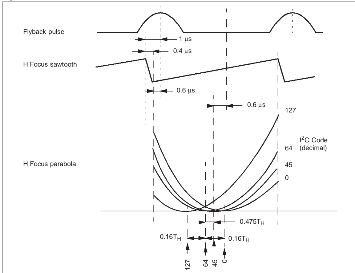
Figure 15. Phase of HFocus Parabola
