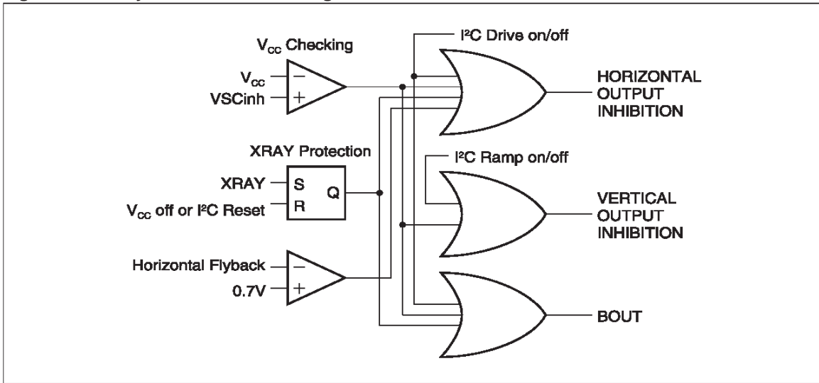
Figure 14. Safety Functions Block Diagram
