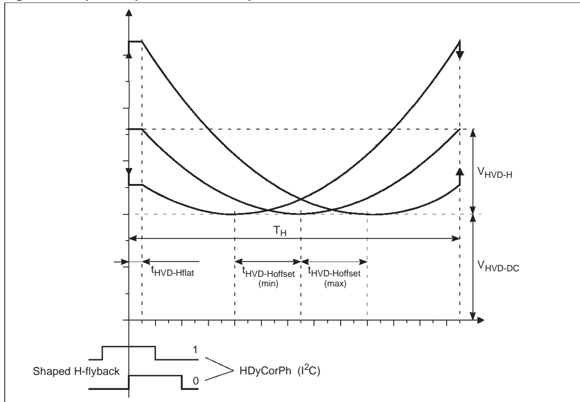
Figure 14. HDyCor output horizontal component waveform
