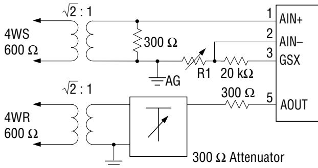
b. Transformer of turns ratio 1 : \sqrt{2}
