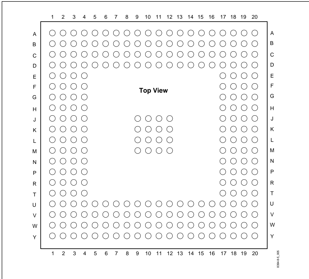
Figure 1-5. CN8398 272-Pinout Diagram
