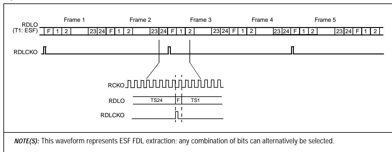
Figure 2-4. Receive External Data Link Waveforms
