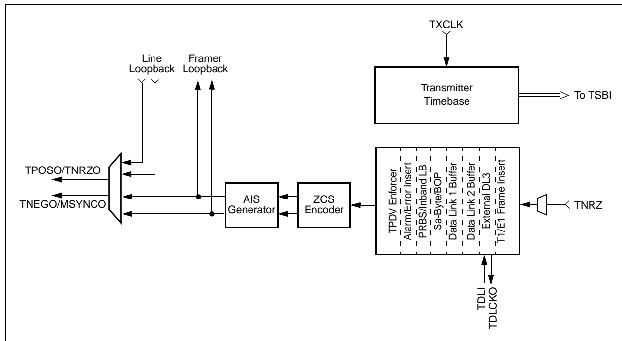
Figure 2-20. XMTR Diagram
