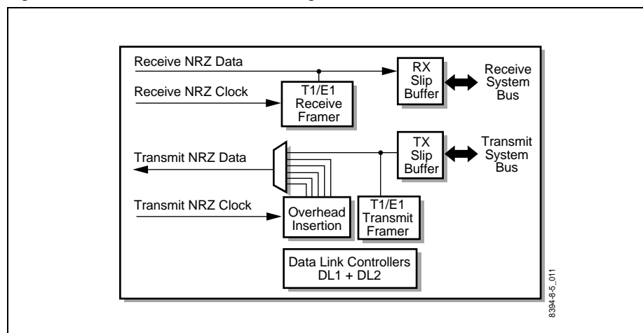
Figure 1-1. CN8395 Functional Block Diagram
