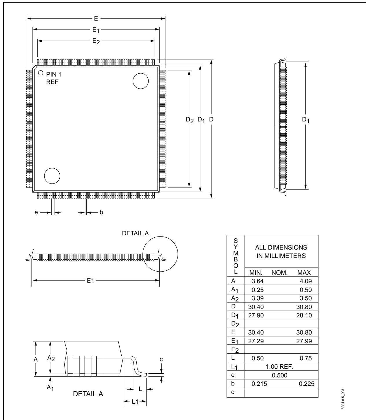
Figure 4-25. 208-Pin Plastic Quad Flat Pack (PQFP)
