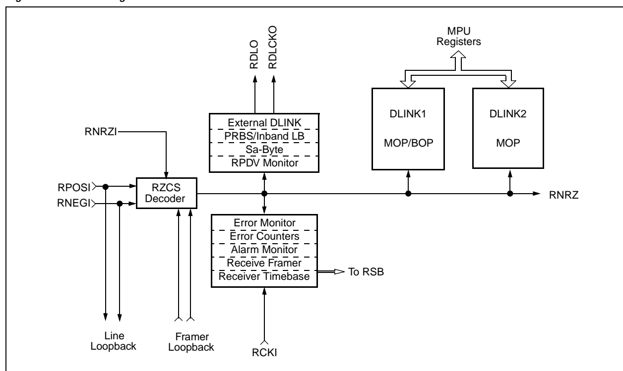
Figure 2-3. RCVR Diagram
