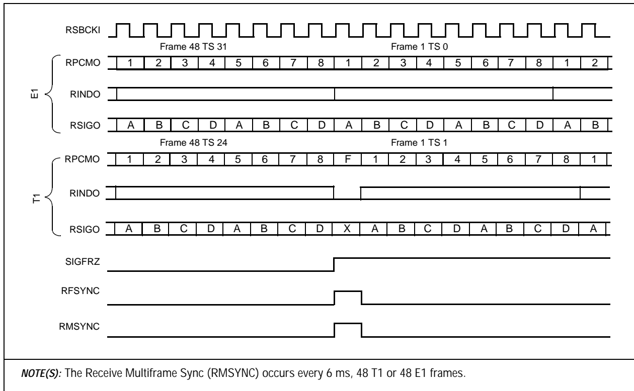
Figure 2-9. RSB Waveforms
