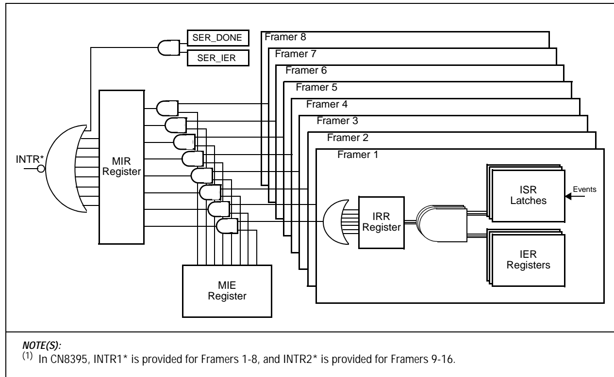
Figure 2-26. Interrupt Generation Block Diagram
