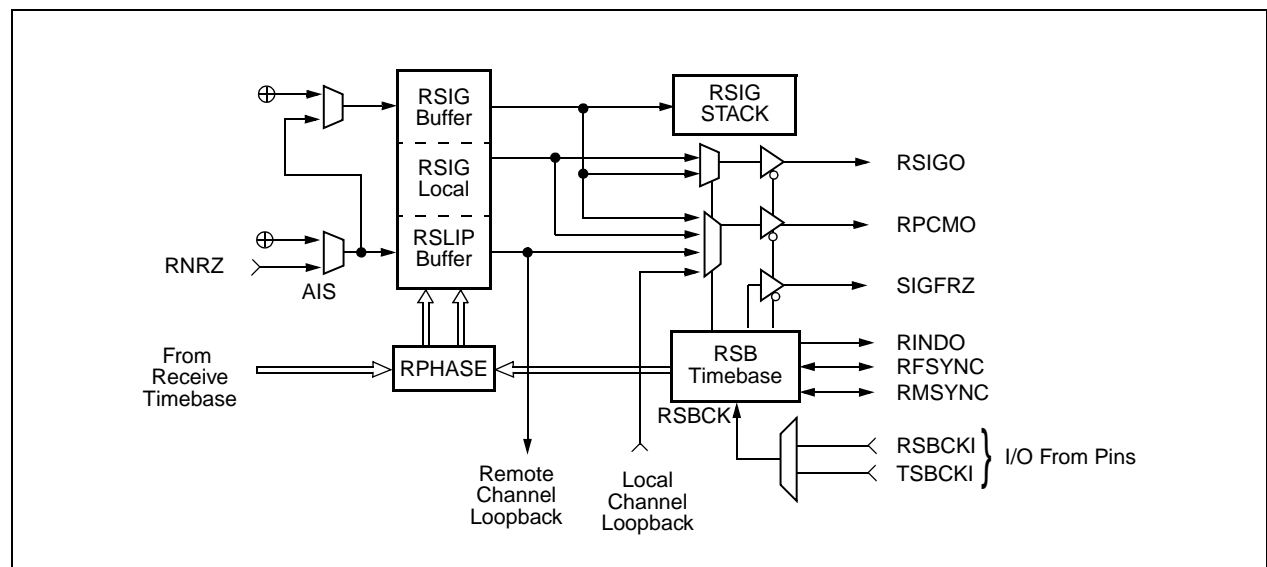
Figure 2-12. RSB Diagram
