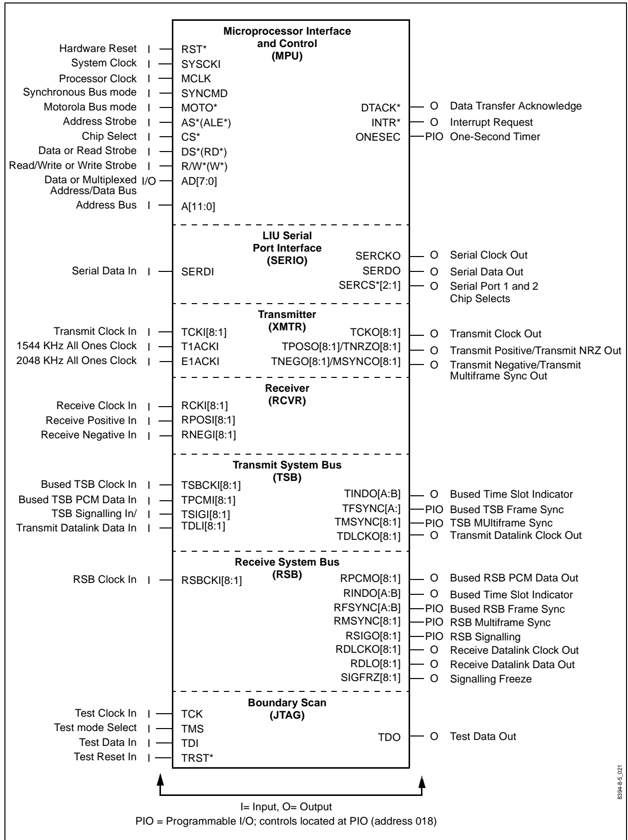
Figure 1-9. CN8398 Logic Diagram (Multiplexed System Bus Mode)
