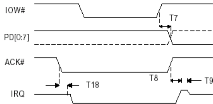
Figure 3. Parallel Port Timing in SPP, PS/2 Mode
