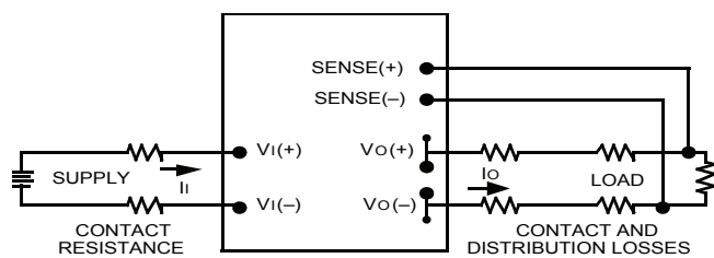
Figure 30. Effective Circuit Configuration for Single-Module Remote-Sense Operation
