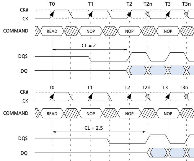
Burst Length = 4 in the cases shown Shown with nominal t_{AC} and nominal t_{DSDQ}
