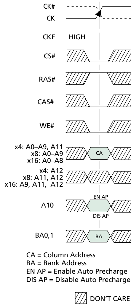
Figure 14 WRITE Command
