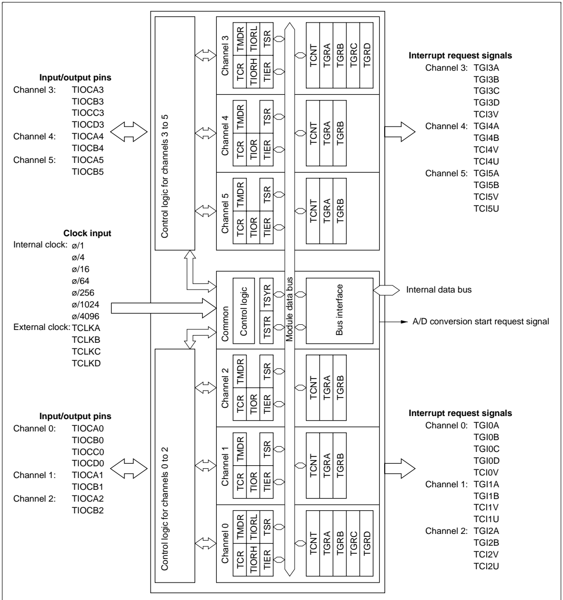
Figure 9-1 Block Diagram of TPU
