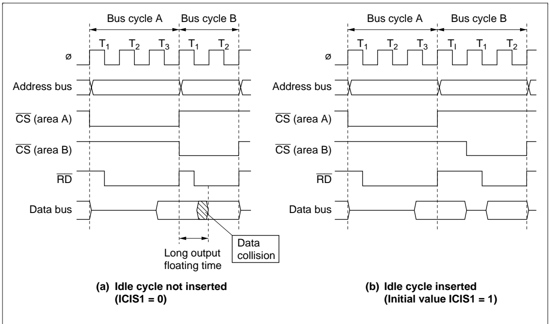
Figure 6-16 Example of Idle Cycle Operation (1)
