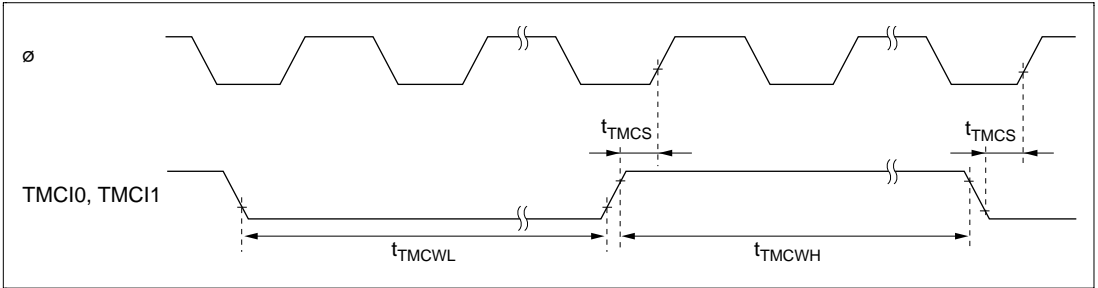
Figure 20-18 8-Bit Timer Clock Input Timing
