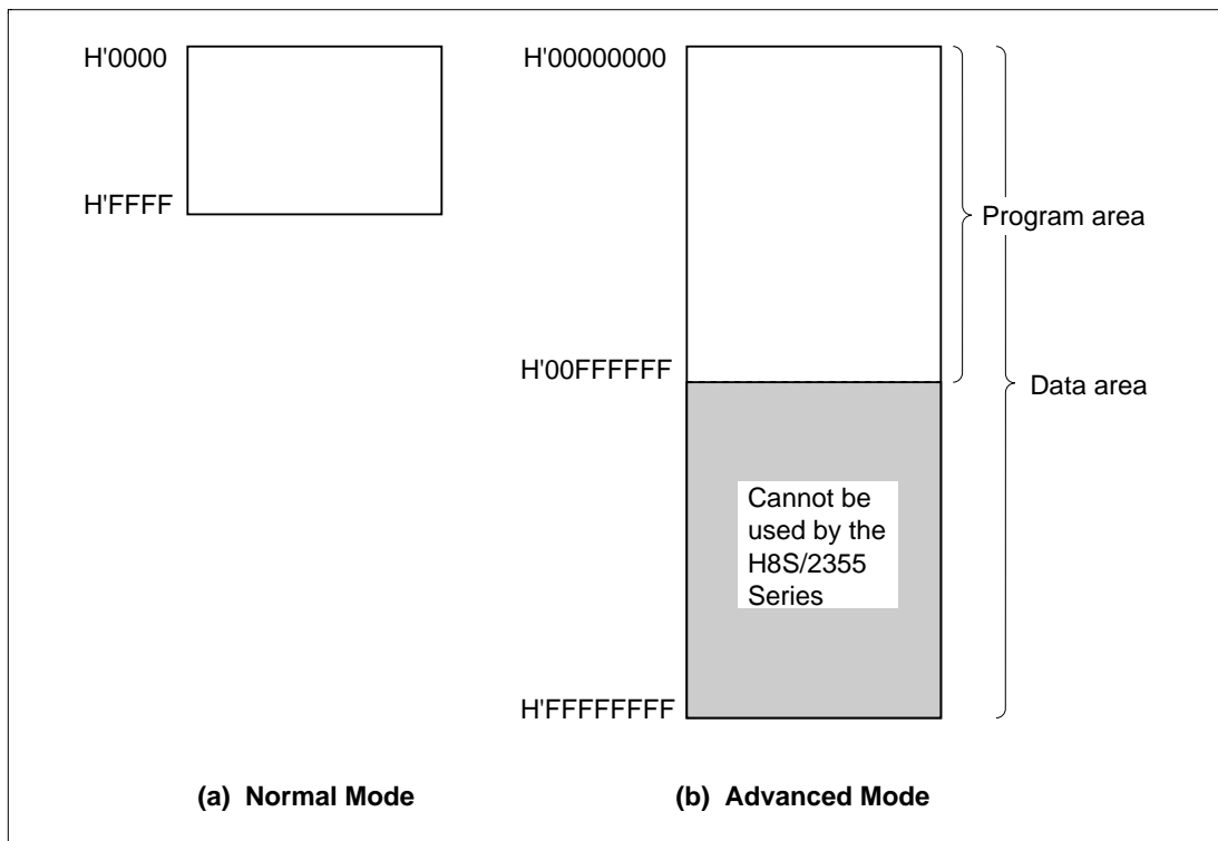
Figure 2-6 Memory Map
