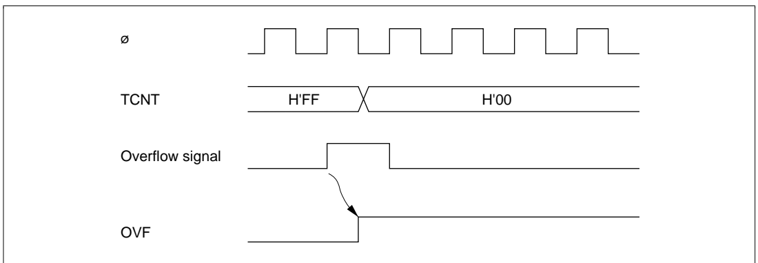
Figure 10-8 Timing of OVF Setting
