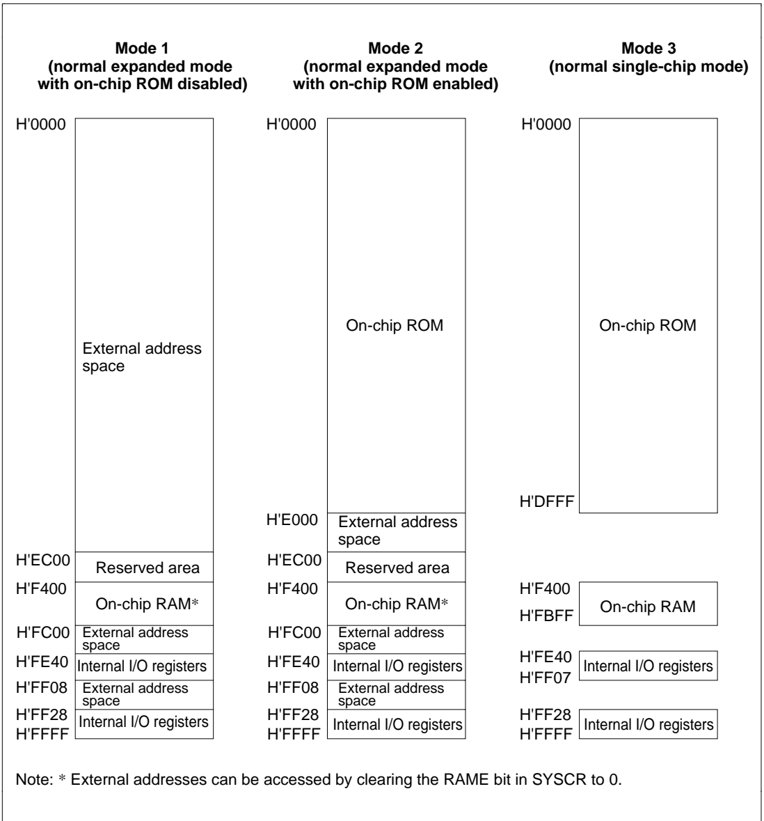
Figure 3-2 Memory Map in Each Operating Mode in the H8S/2353
