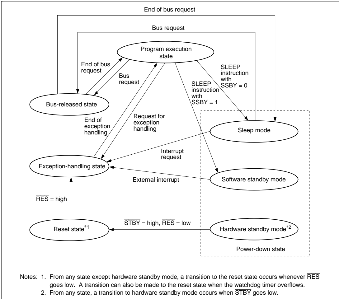
Figure 2-15 State Transitions
