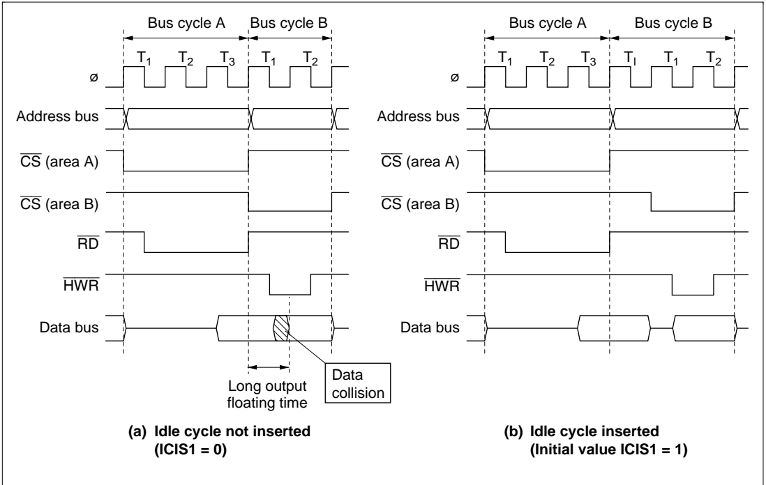
Figure 6-17 Example of Idle Cycle Operation (2)
