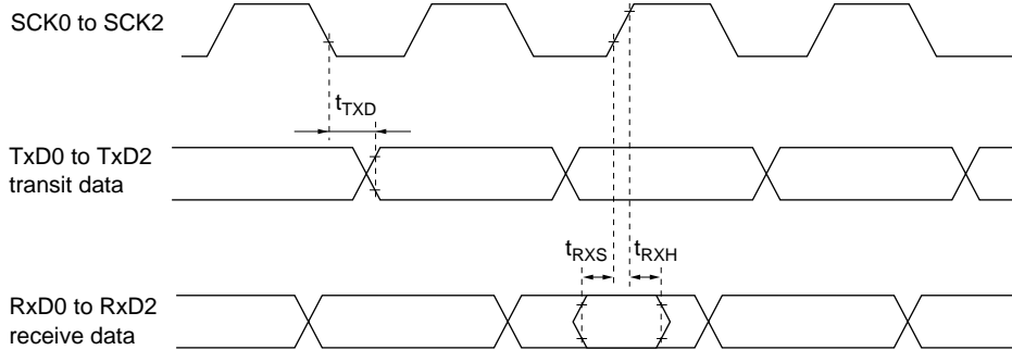
Figure 20-22 SCI Input/Output Timing (Clock Synchronous Mode)
