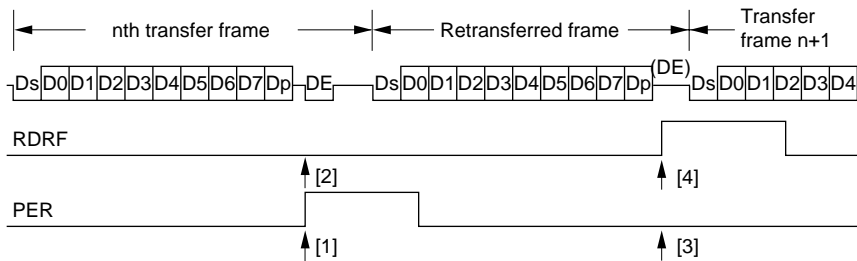
Figure 13-11 Retransfer Operation in SCI Receive Mode
