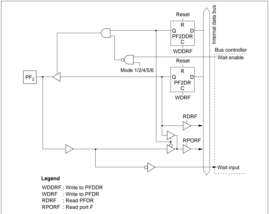
Figure C-12 (c) Port F Block Diagram (Pin PF 2 )
