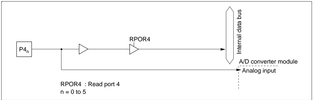
Figure C-4 (a) Port 4 Block Diagram (Pins P4_0 to P4_5 in H8S/2355 and H8S/2353, Pins P4_0 to P4_7 in H8S/2393)
