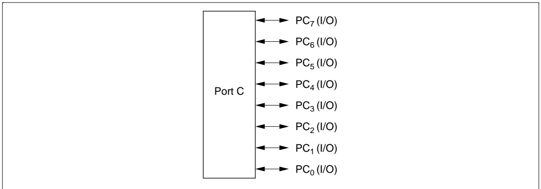
Figure 8-18 Port C Pin Functions (Modes 3 and 7)
