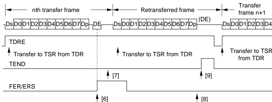
Figure 13-12 Retransfer Operation in SCI Transmit Mode
