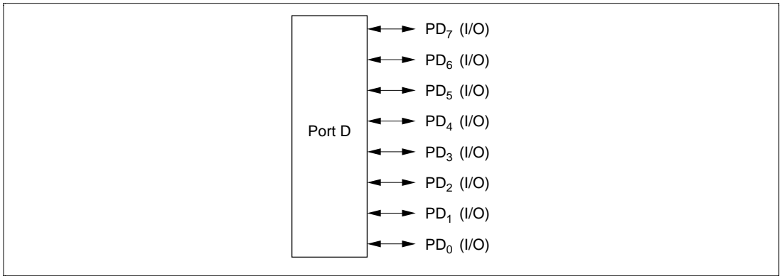
Figure 8-21 Port D Pin Functions (Modes 3 and 7)
