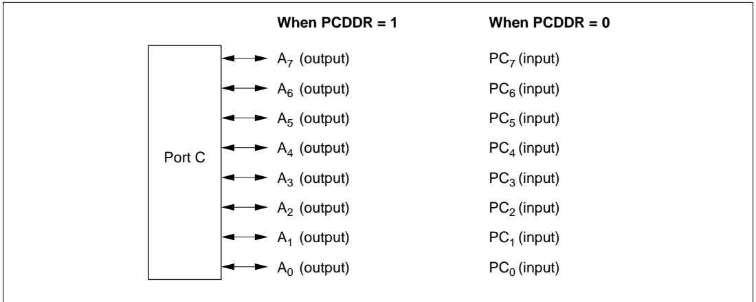
Figure 8-17 Port C Pin Functions (Modes 2 and 6)
