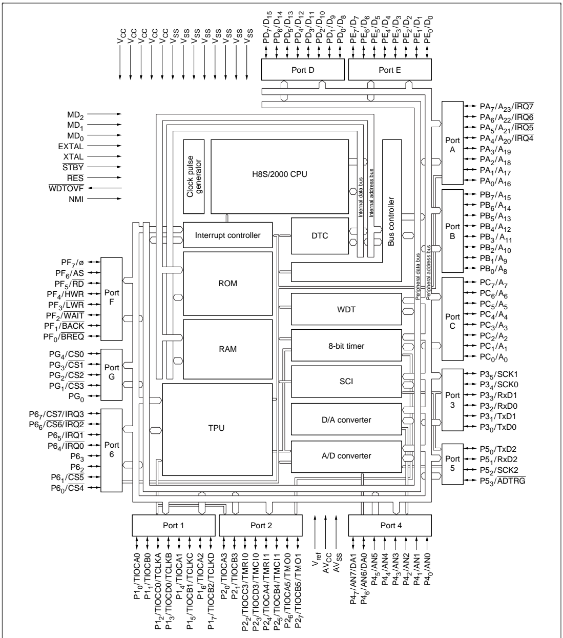
Figure 1-1 Block Diagram (H8S/2355, H8S/2353)
