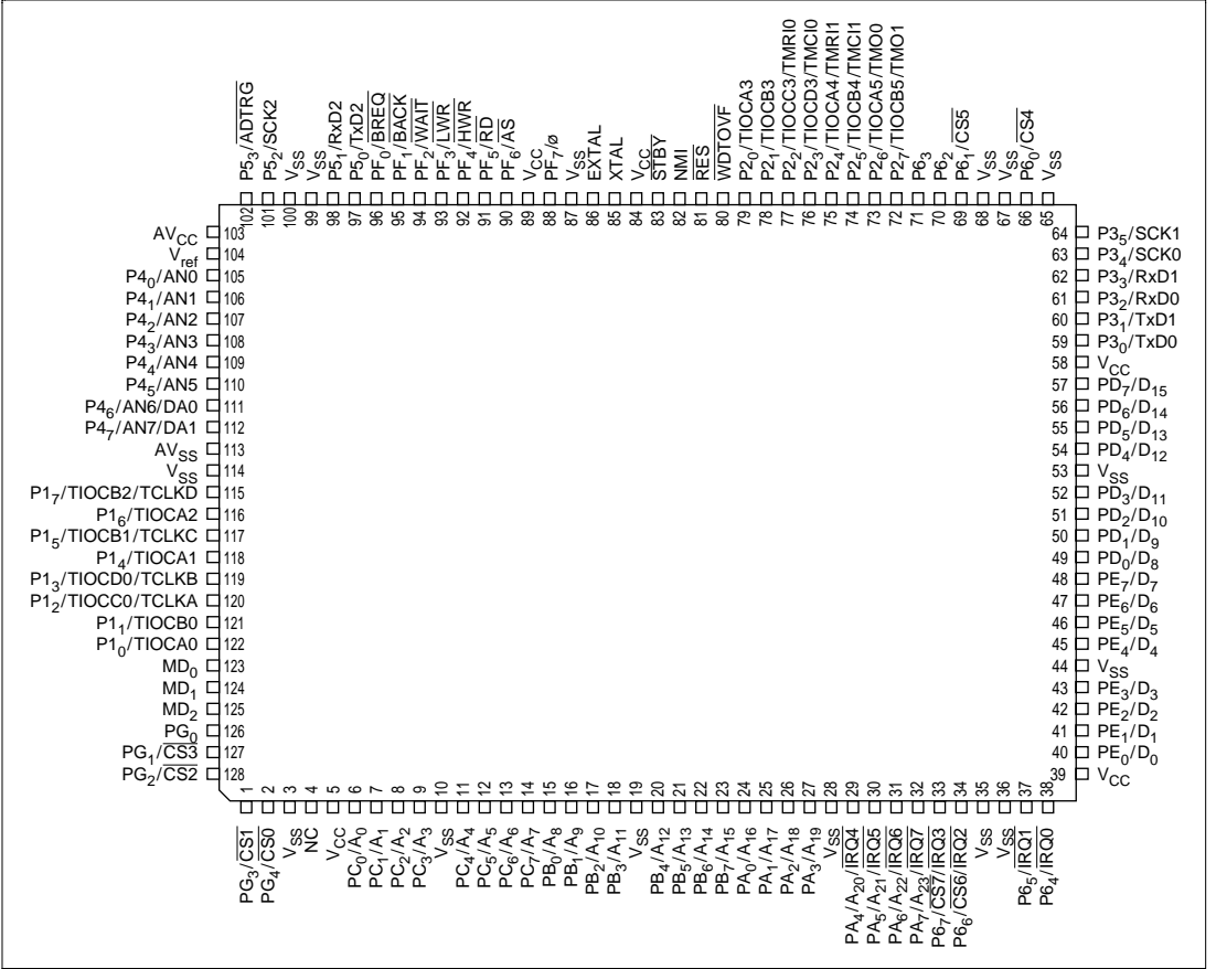
Figure 1-4 H8S/2355 and H8S/2353 Pin Arrangement (FP-128: Top View)
