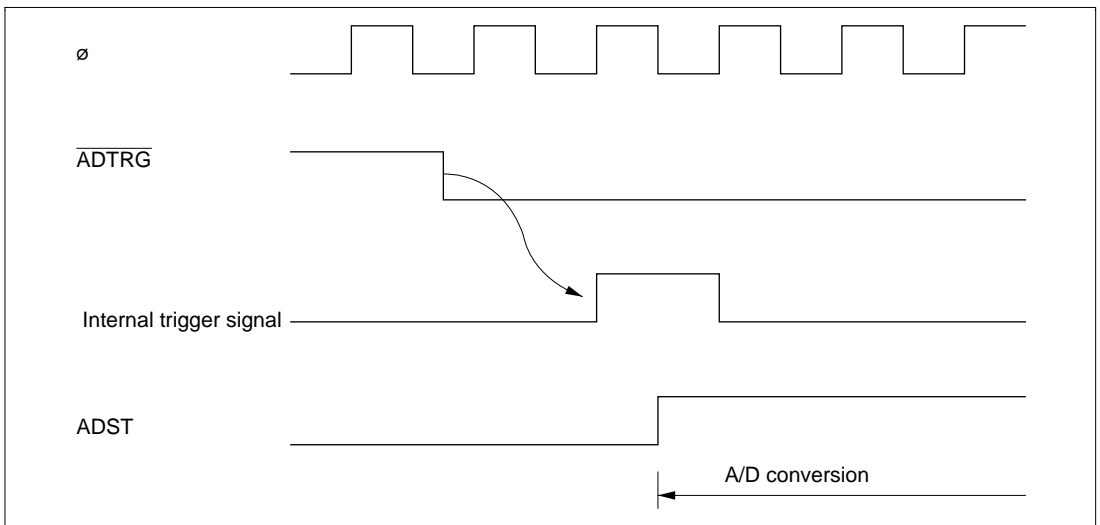
Figure 14-6 External Trigger Input Timing
