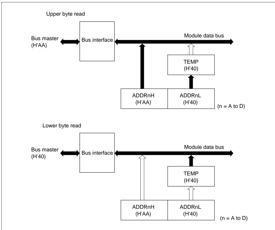
Figure 14-2 ADDR Access Operation (Reading H'AA40)
