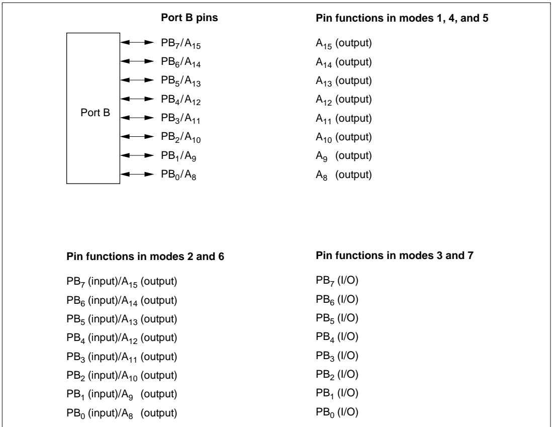
Figure 8-11 Port B Pin Functions
