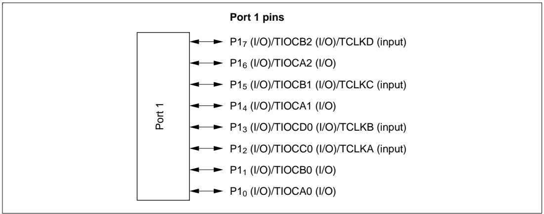
Figure 8-1 Port 1 Pin Functions
