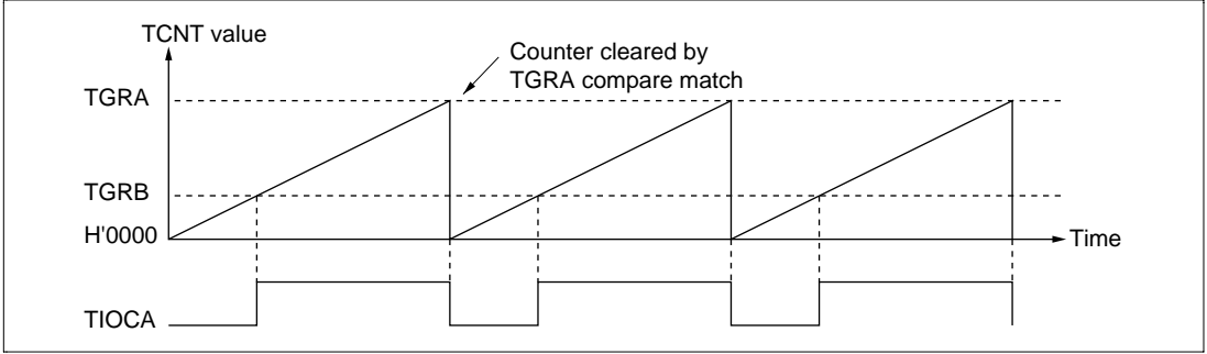
Figure 9-25 Example of PWM Mode Operation (1)
