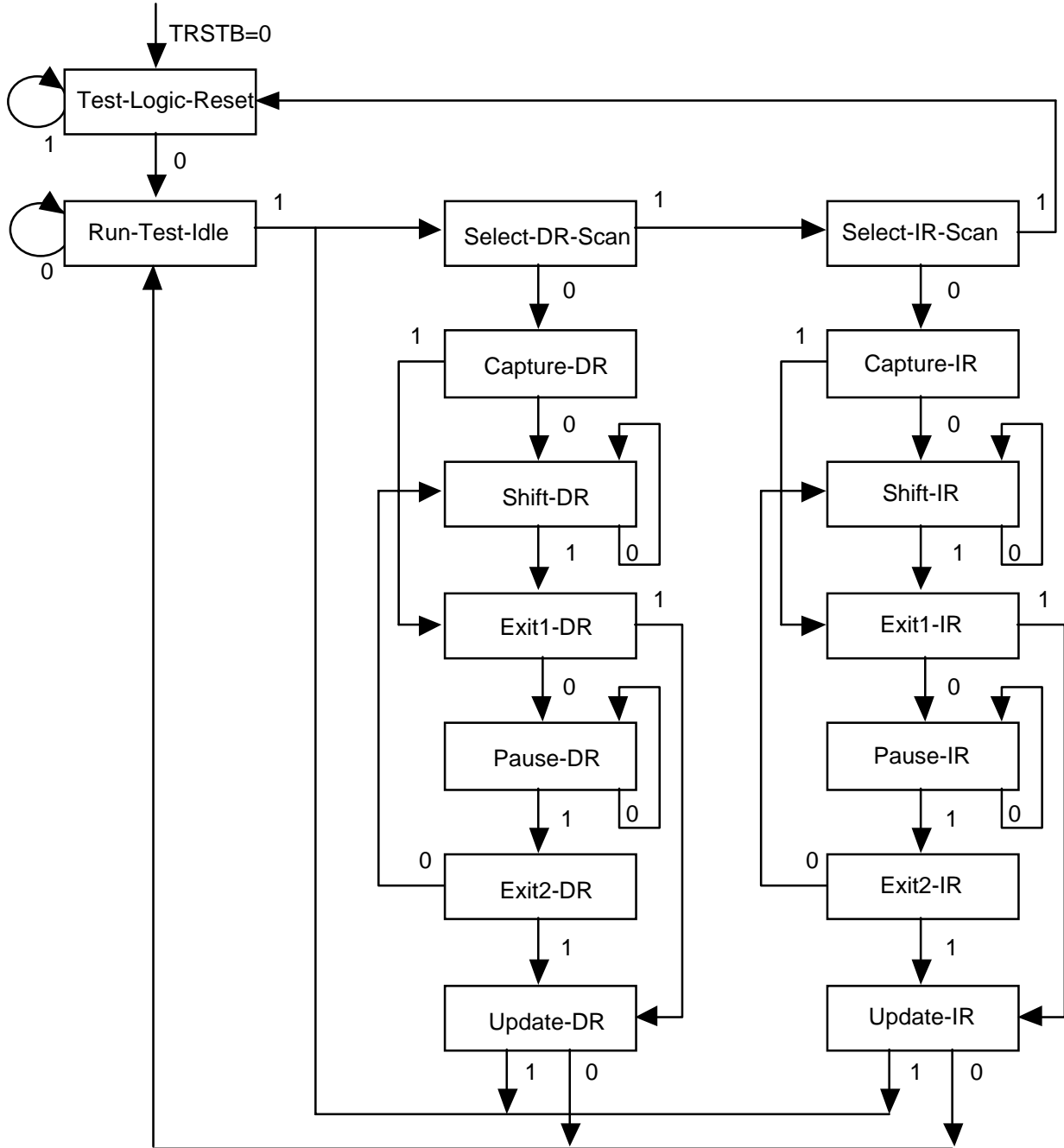
Fig. 9 TAP Controller Finite State Machine
