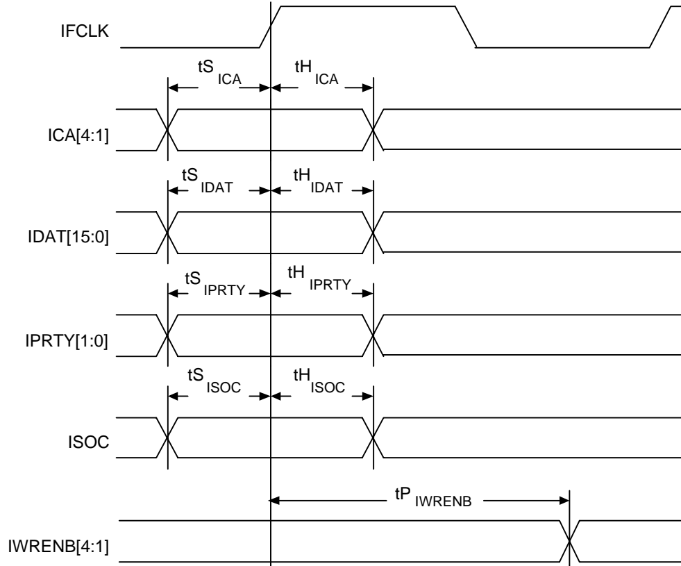
Fig. 17 Input Cell Interface Master (IPOLL=0) Timing
