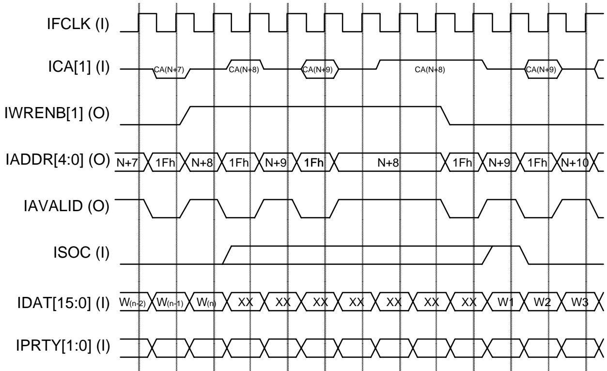
Fig. 12 Input Cell Interface Address Line Polling Master Configuration (IPOLL=1) – Example 2
