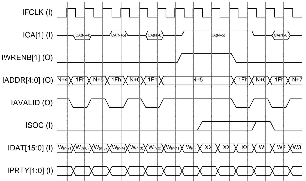
Fig. 11 Input Cell Interface Address Line Polling Master Configuration (IPOLL=1) – Example 1
