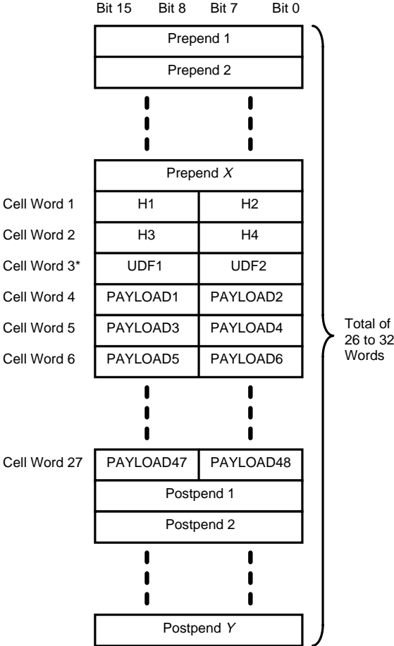
Fig. 7 Sixteen Bit Wide Cell Format
