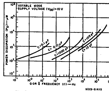
Fig. 31 - Power dissipation vs output frequency ( V_{DD} = 10 V).
