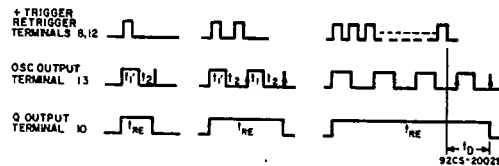
Fig. 29 - Retrigger-mode waveforms.
