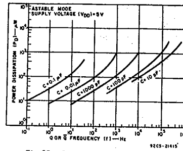
Fig. 30 - Power dissipation vs output frequency ( V_{DD} = 5 V).
