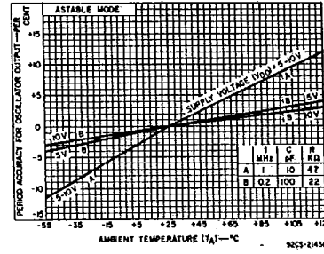
Fig. 20 — Typical oscillator-period accuracy vs temperature (high frequency).
