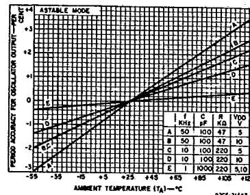
Fig. 17 - Typical Q-and-Q-bar-period accuracy vs temperature (medium frequency).
