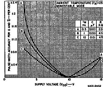
Fig. 23 — Typical Q- and Q̄-pulse-width accuracy vs supply voltage (t M = 0.5, 1, 10 ms).
