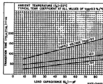
Fig. 7 - Typical transition time vs load capacitance for Q and \bar{Q} buffers.
