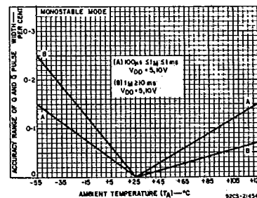
Fig. 27 — Typical Q and Q̄ pulse-width accuracy range vs temperature.
