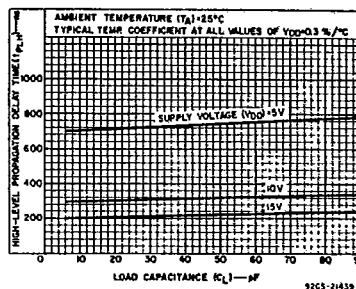
Fig. 6 - Typical low-to-high level propagation delay time vs load capacitance for Q and \bar{Q} buffers.
