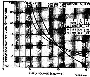
Fig. 10 - Typical Q-and-Q-bar-period accuracy vs supply voltage (high frequency).
