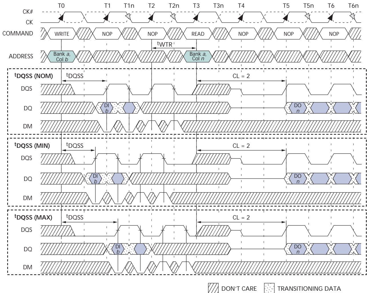
Figure 41: WRITE-to-READ - Interrupting
