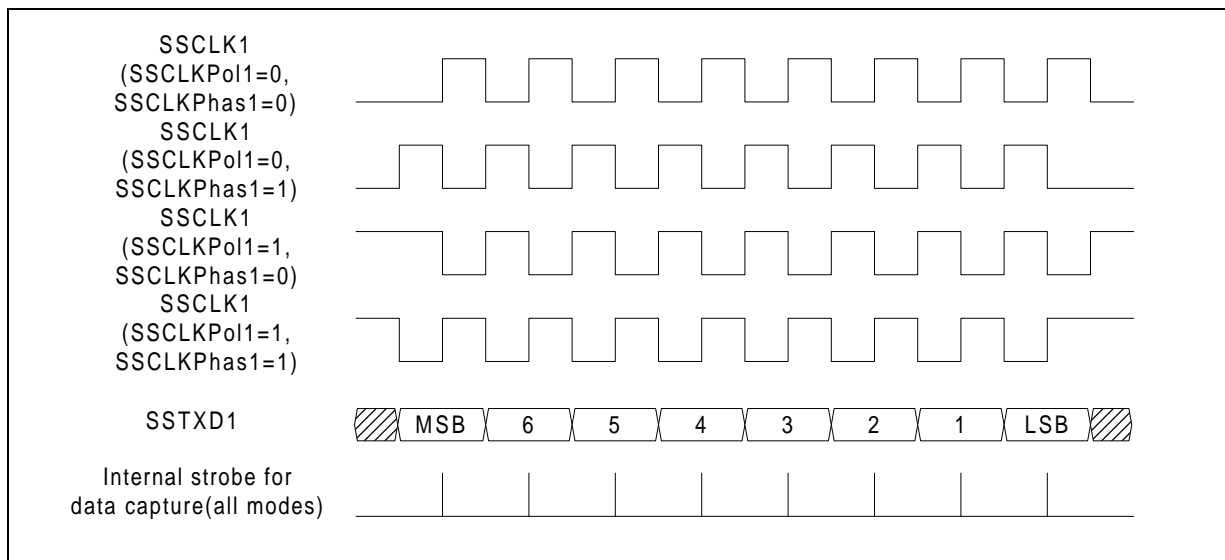
Figure 19-2. SSCLK1 Diagram
