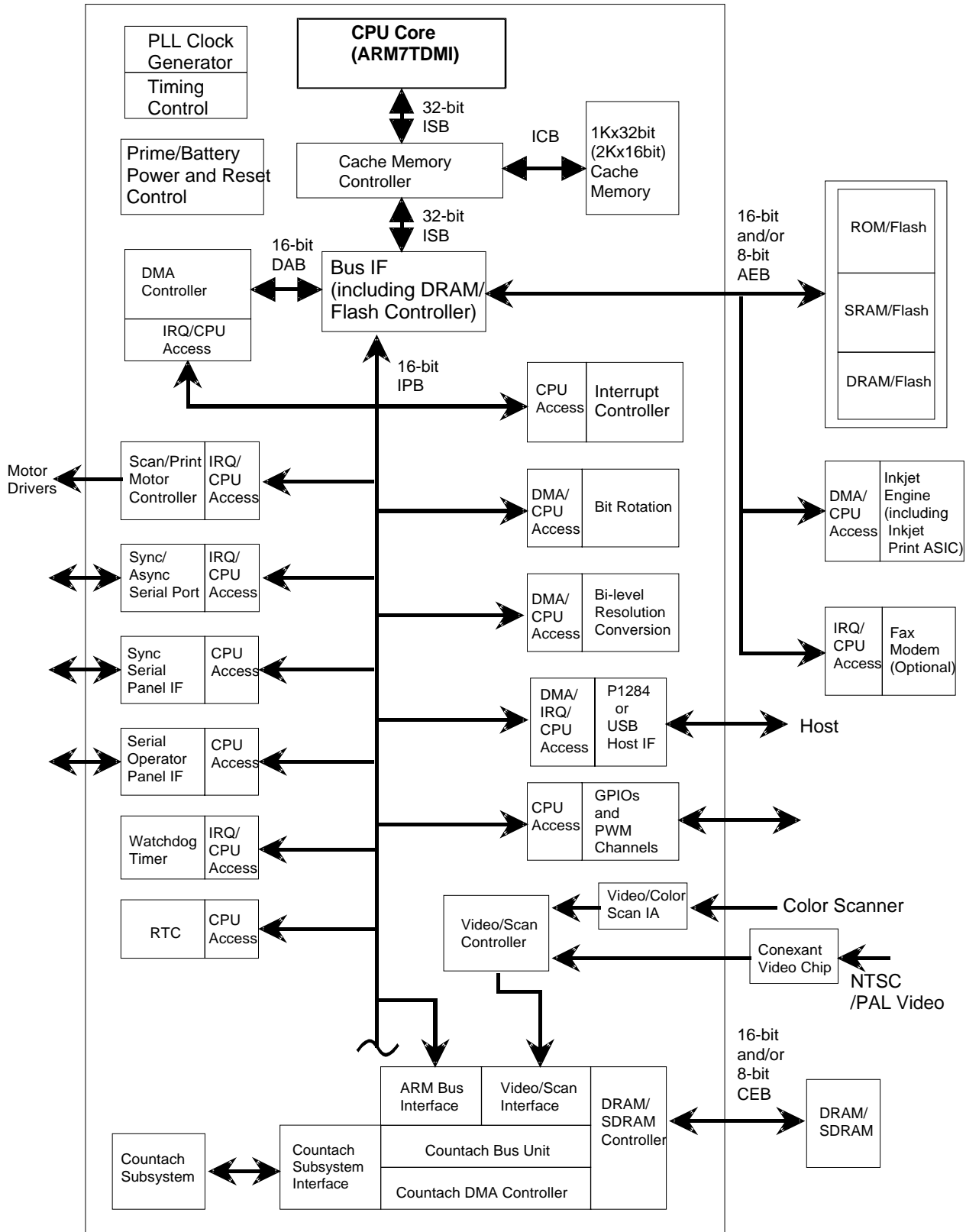
Figure 2-1. MFC2000 Organization
