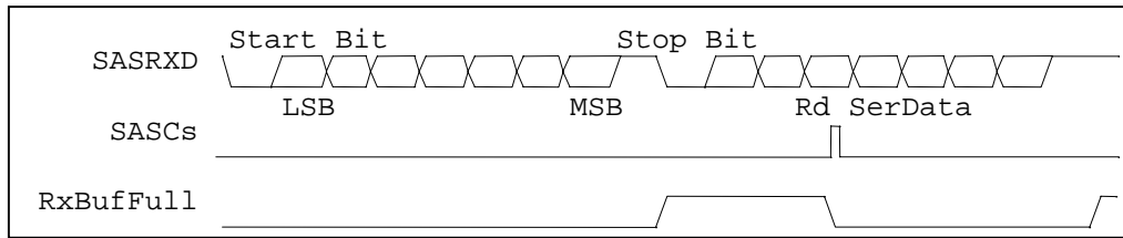
Figure 15-7. Asynchronous Receiver Byte Timing – FIFO mode disabled
