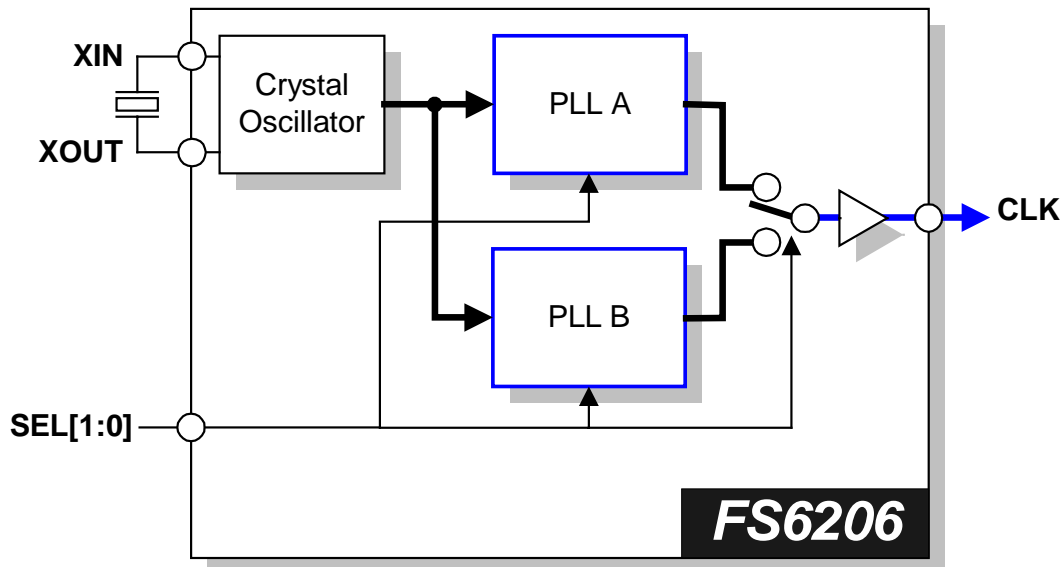
Figure 2: Block Diagram
