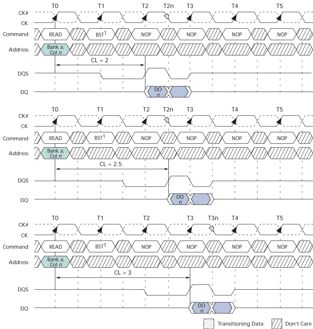
Figure 32: Terminating a READ Burst
