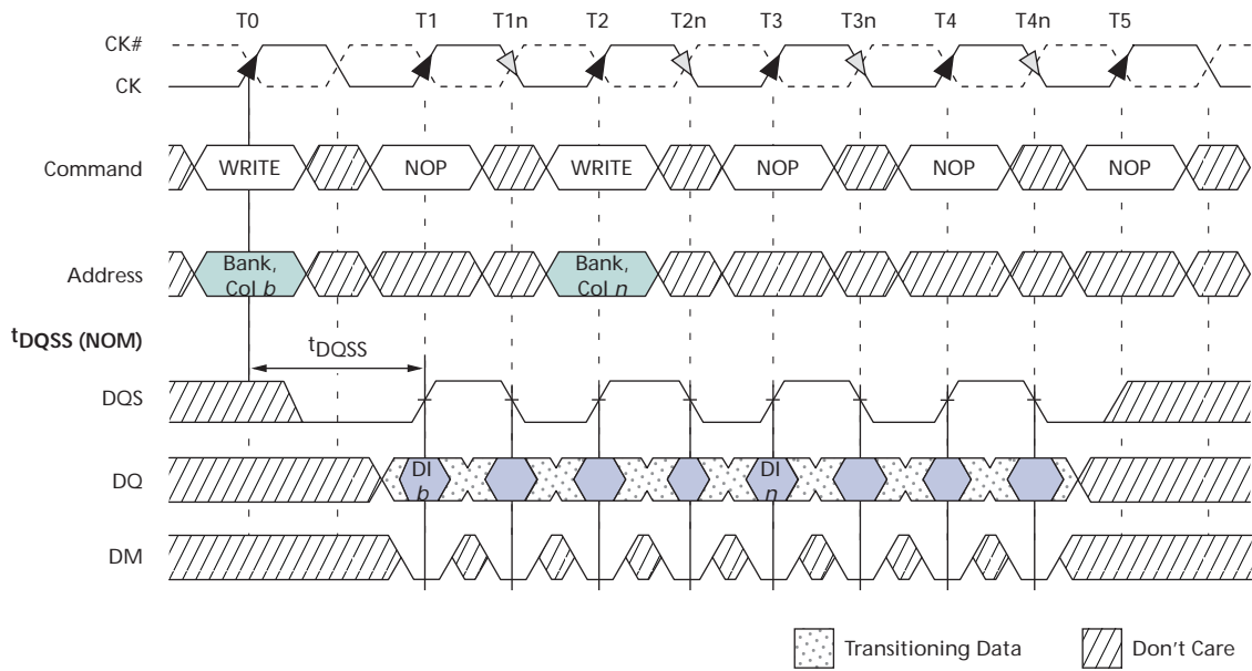
Figure 40: Consecutive WRITE-to-WRITE
