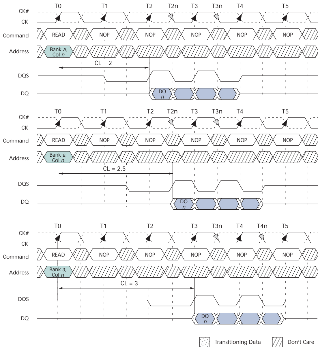
Figure 28: READ Burst
