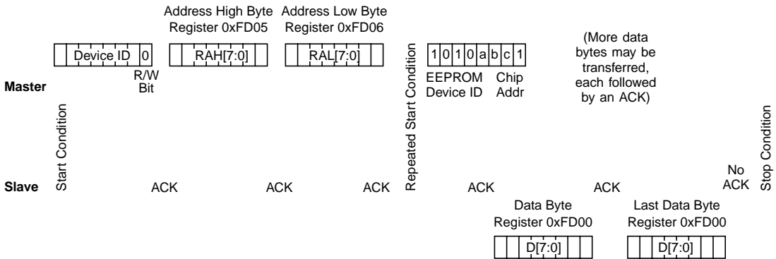
Figure 2.10 Serial ROM Download
