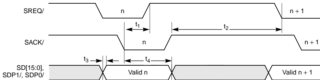
Figure 9.20 Target Asynchronous Receive Waveforms
