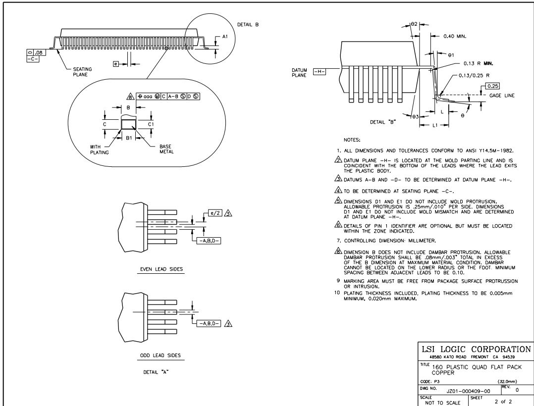
Figure 9.21 160-Lead PQFP (P3) Mechanical Drawing (Sheet 2 of 2)
