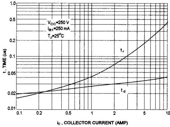
TURN-ON TIME
