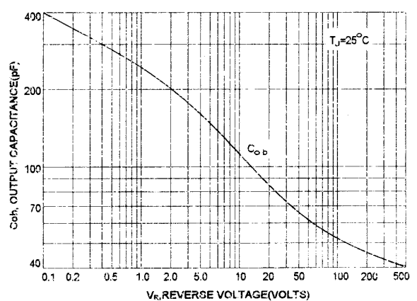
OUTPUT CAPACITANCES
