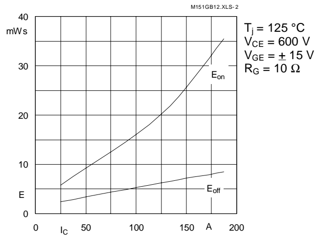
Fig. 2 Turn-on /-off energy E = f(I_C)
