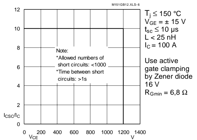
Fig. 6 Safe operating area at short circuit I_{Csc} = f(V_{CE})
