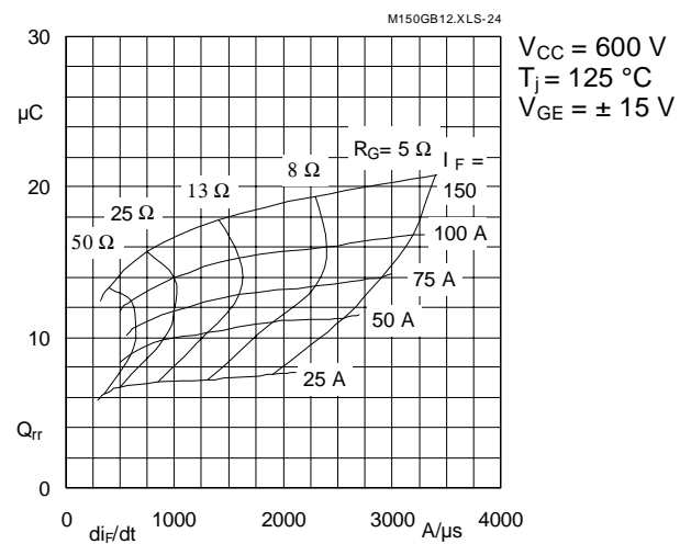
Fig. 24 Typ. CAL diode recovered charge Q_{rr} = f(di/dt)
