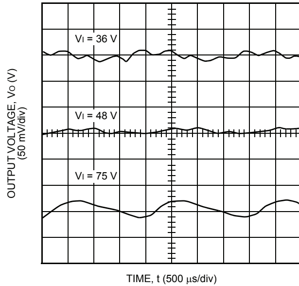
Figure 15. Typical JW100R Output Ripple Voltage at Room Temperature, 36 Vdc to 75 V Input, and 2.7 A Output
