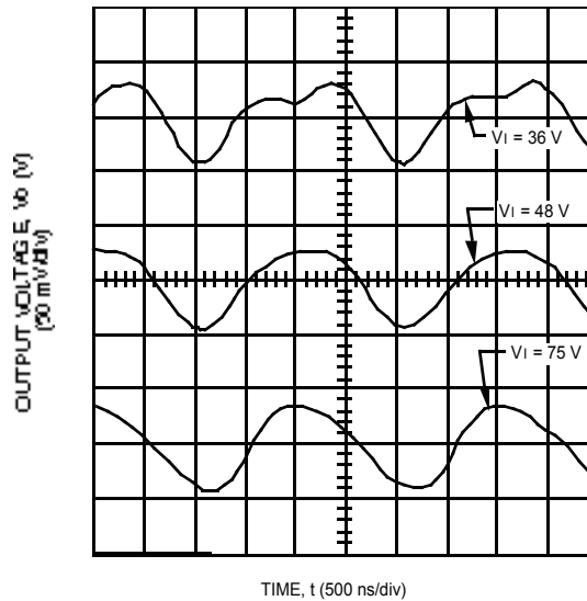
Figure 16. Typical JW150R Output Ripple Voltage at Room Temperature, 36 Vdc to 75 V Input, and 5.4 A Output
