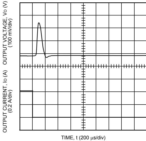
8-2722 (F) Note: Tested with a 10 \mu F aluminum and a 1.0 \mu F ceramic capacitor across the load.
