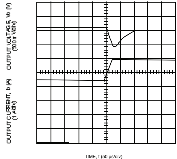
8-1881 (C) Note: Tested with a 10 \mu F aluminum and a 1.0 \mu F ceramic capacitor across the load.
