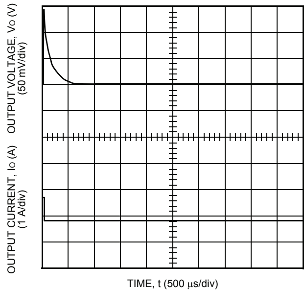
8-2723 (F) Note: Tested with a 10 \mu F aluminum and a 1.0 \mu F ceramic capacitor across the load.
