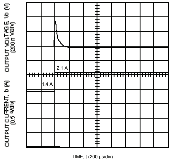
8-2128 (C) Note: Tested with a 10 \mu F aluminum and a 1.0 \mu F ceramic capacitor across the load.
