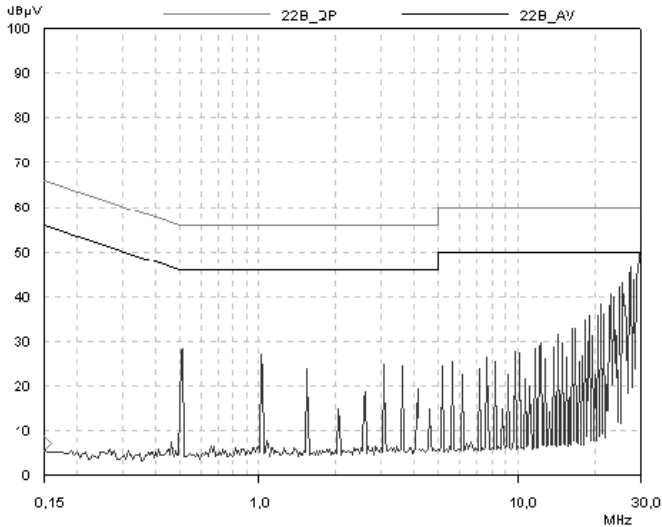
PKF 4928A with 51µH common mode and 10 µH series inductor
