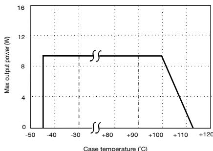
Power derating
