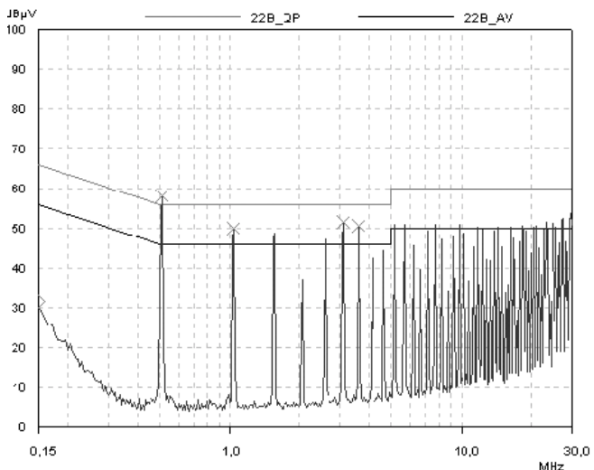
PKF 4928 A without filter
