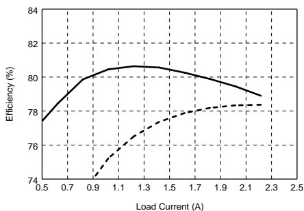
Efficiency (typ) @ T A = +25°C
