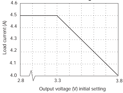
Current derating
