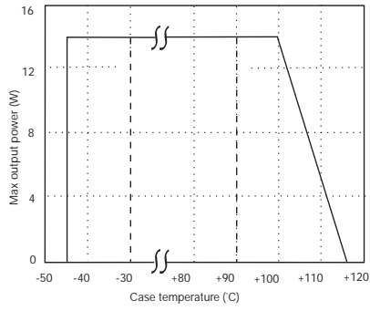
Power derating
