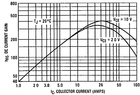
FIGURE 6 — DC CURRENT GAIN
