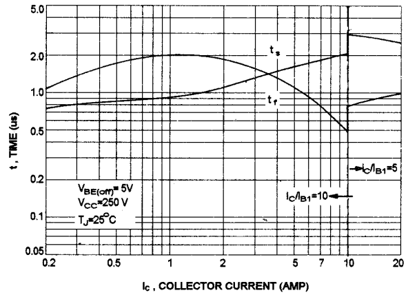
TURN-OFF TIME
