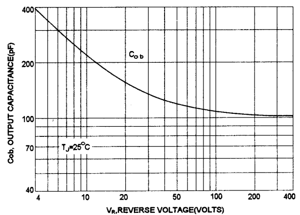
OUTPUT CAPACITANCES
