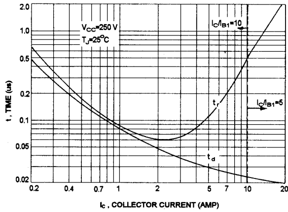
TURN-ON TIME
