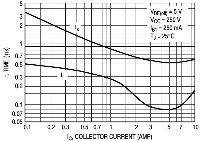
Figure 9. Turn-Off Time
