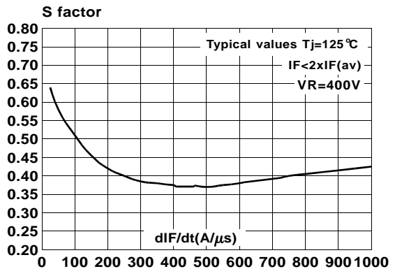
Fig. 6: Softness factor (tb/ta) versus dI/dt.
