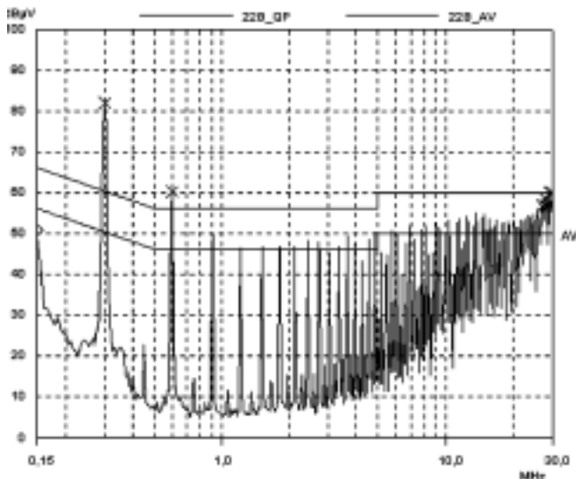
PKF 4910A without filter.
