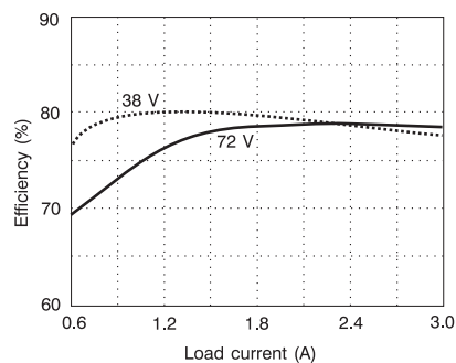
Efficiency (typ) @ T A = +25°C
