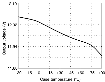
Temperature coefficient
