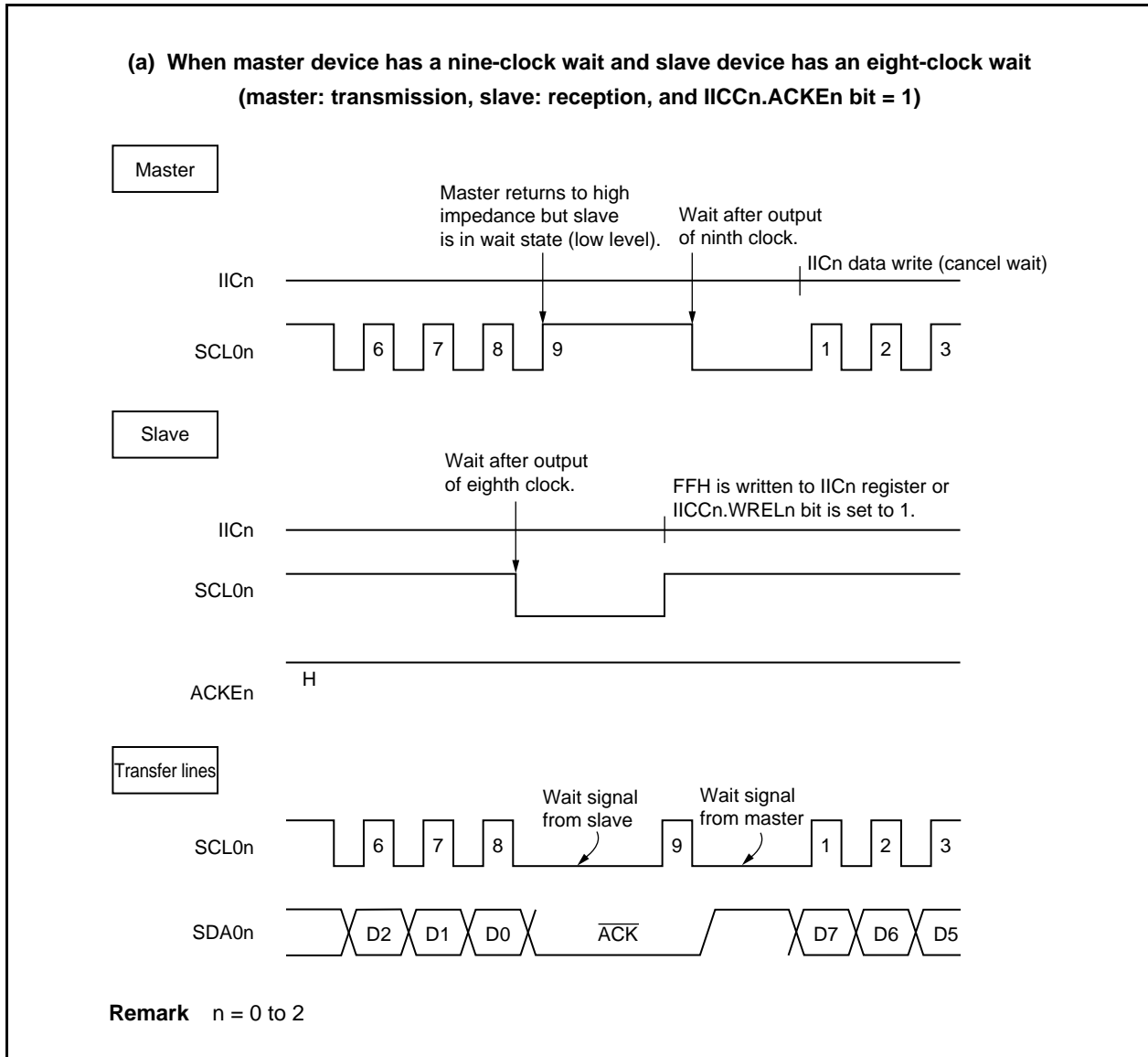
Figure 17-13. Wait Signal (1/2)
