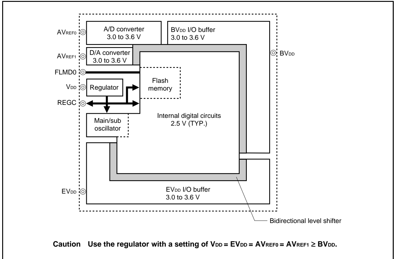
Figure 28-1. Regulator
