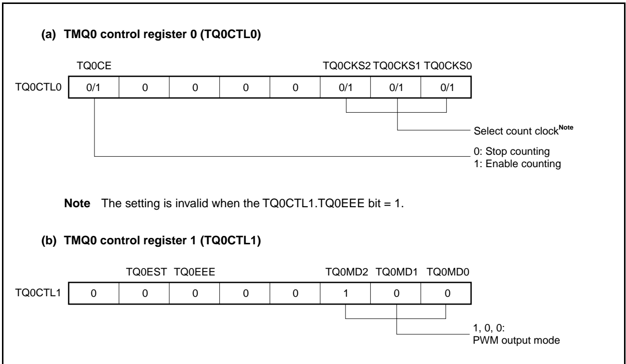
Figure 8-26. Setting of Registers in PWM Output Mode (1/3)
