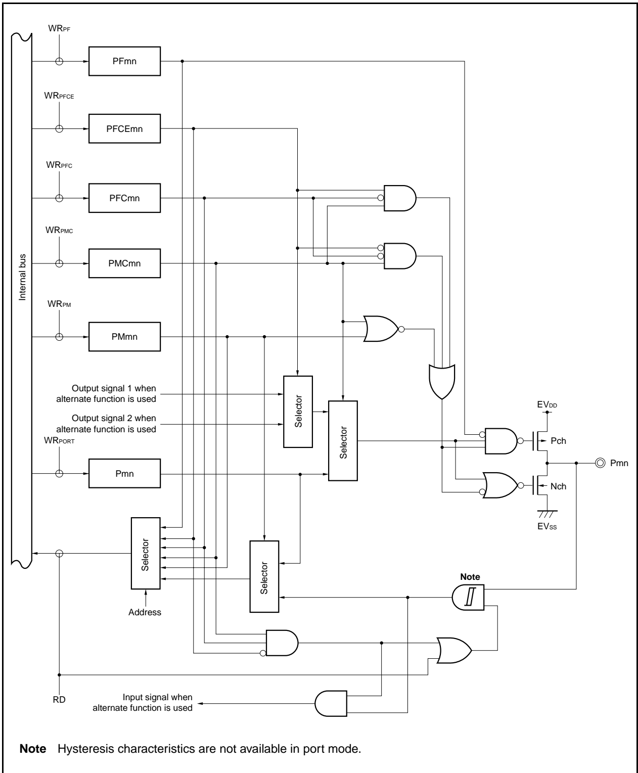
Figure 4-35. Block Diagram of Type U-12
