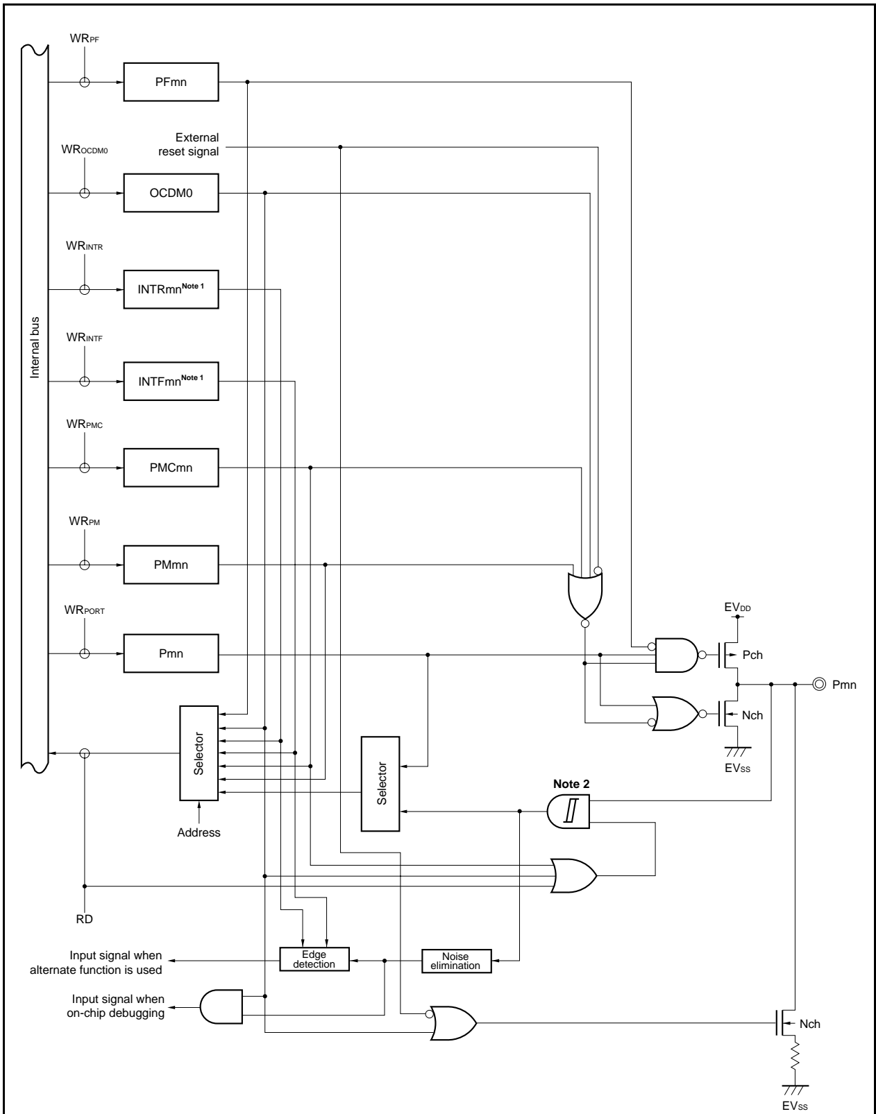
Figure 4-39. Block Diagram of Type AA-1
