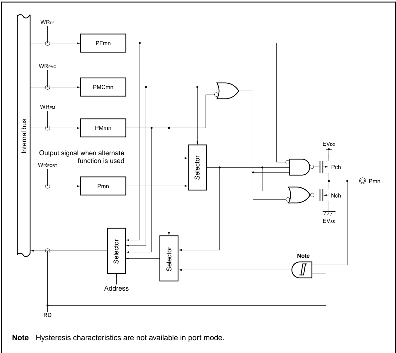
Figure 4-11. Block Diagram of Type E-2
