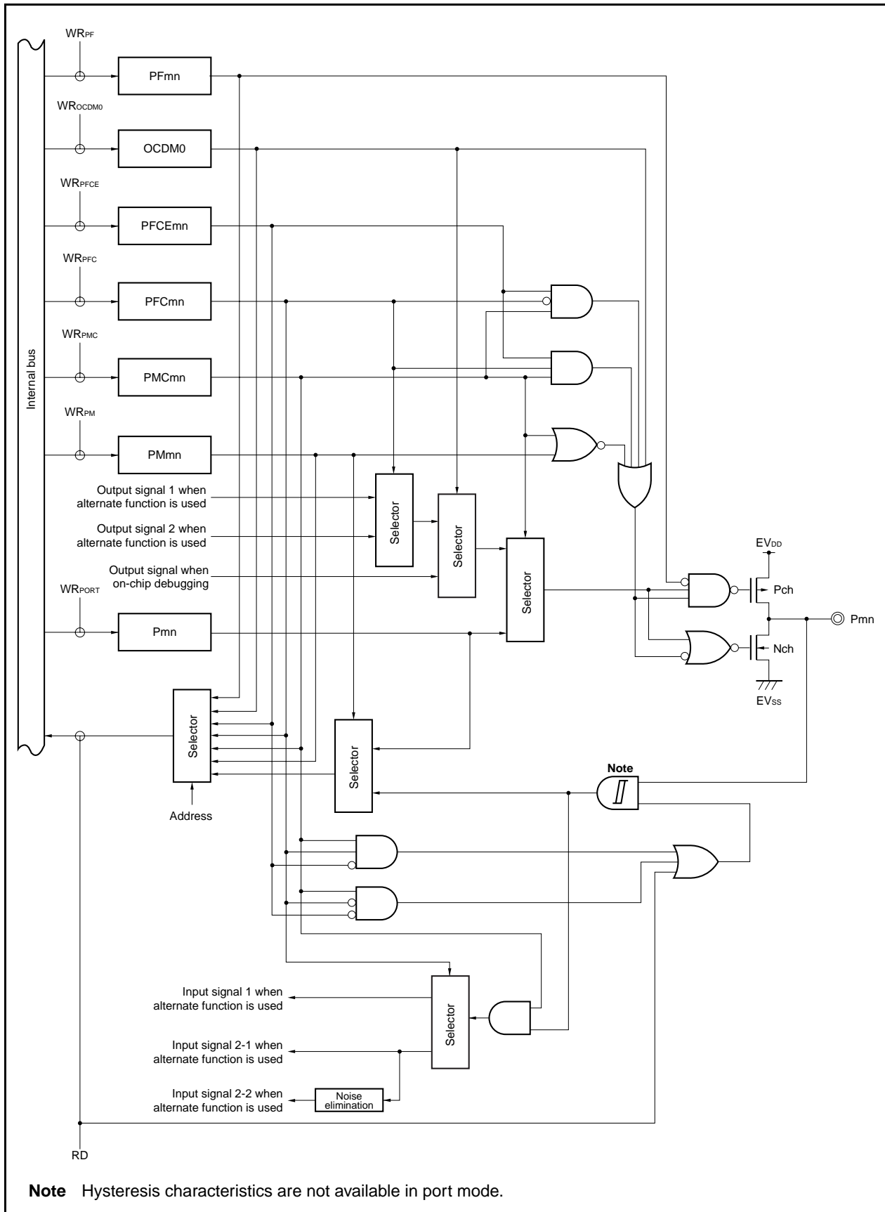
Figure 4-30. Block Diagram of Type U-7
