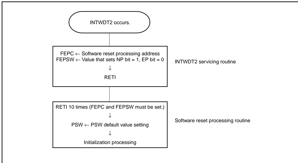
Figure 22-4. Software Reset Processing
