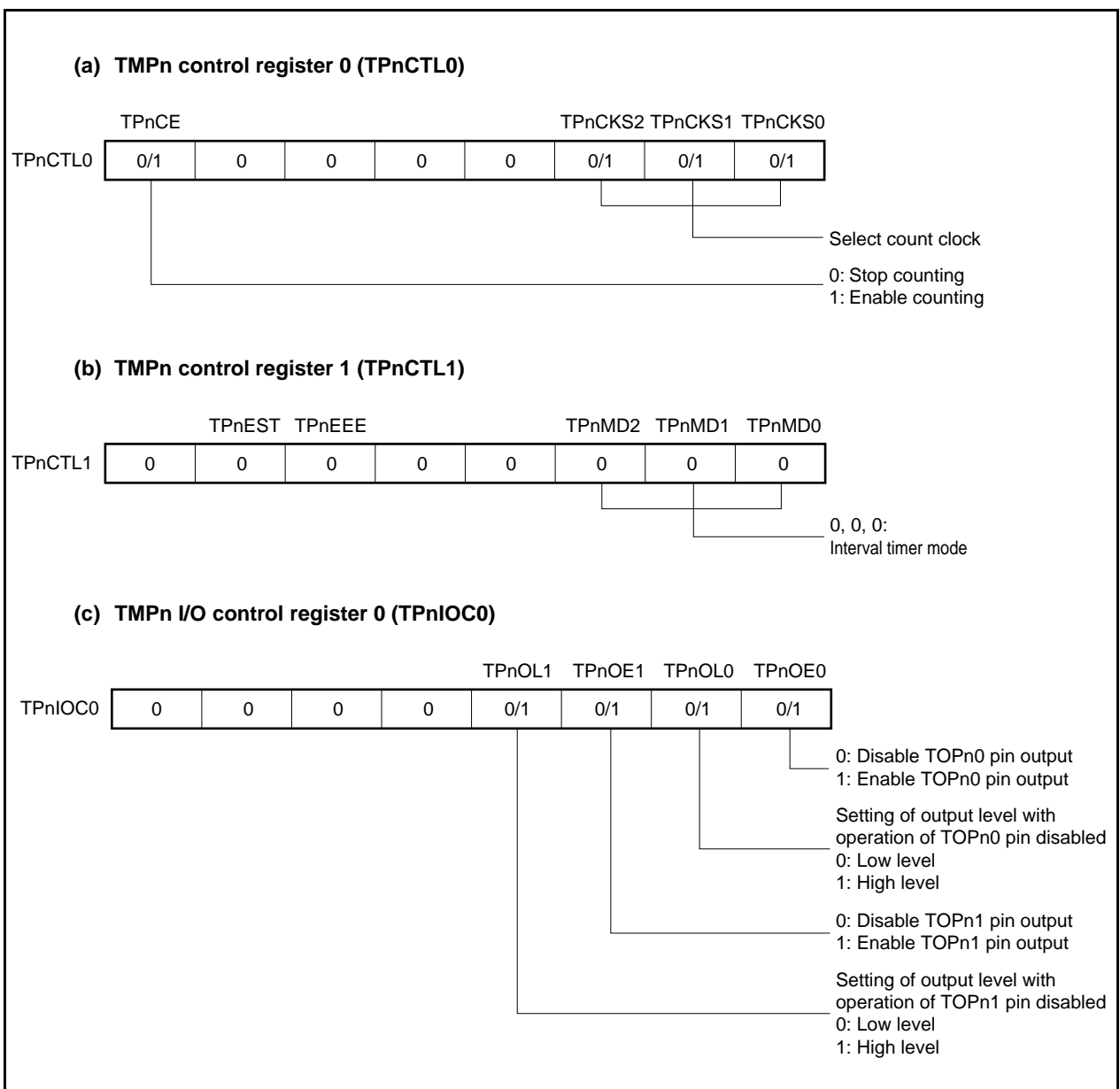
Figure 7-4. Register Setting for Interval Timer Mode Operation (1/2)
