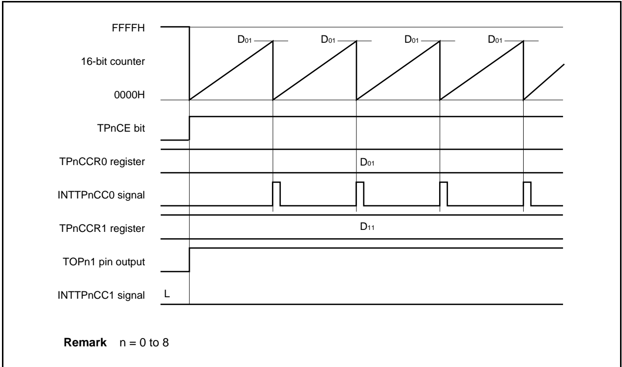
Figure 7-15. Timing Chart When D_{01} < D_{11}
