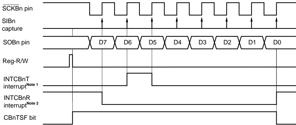
(ii) Communication type 2 (CBnCKP = 0, CBnDAP = 1)
