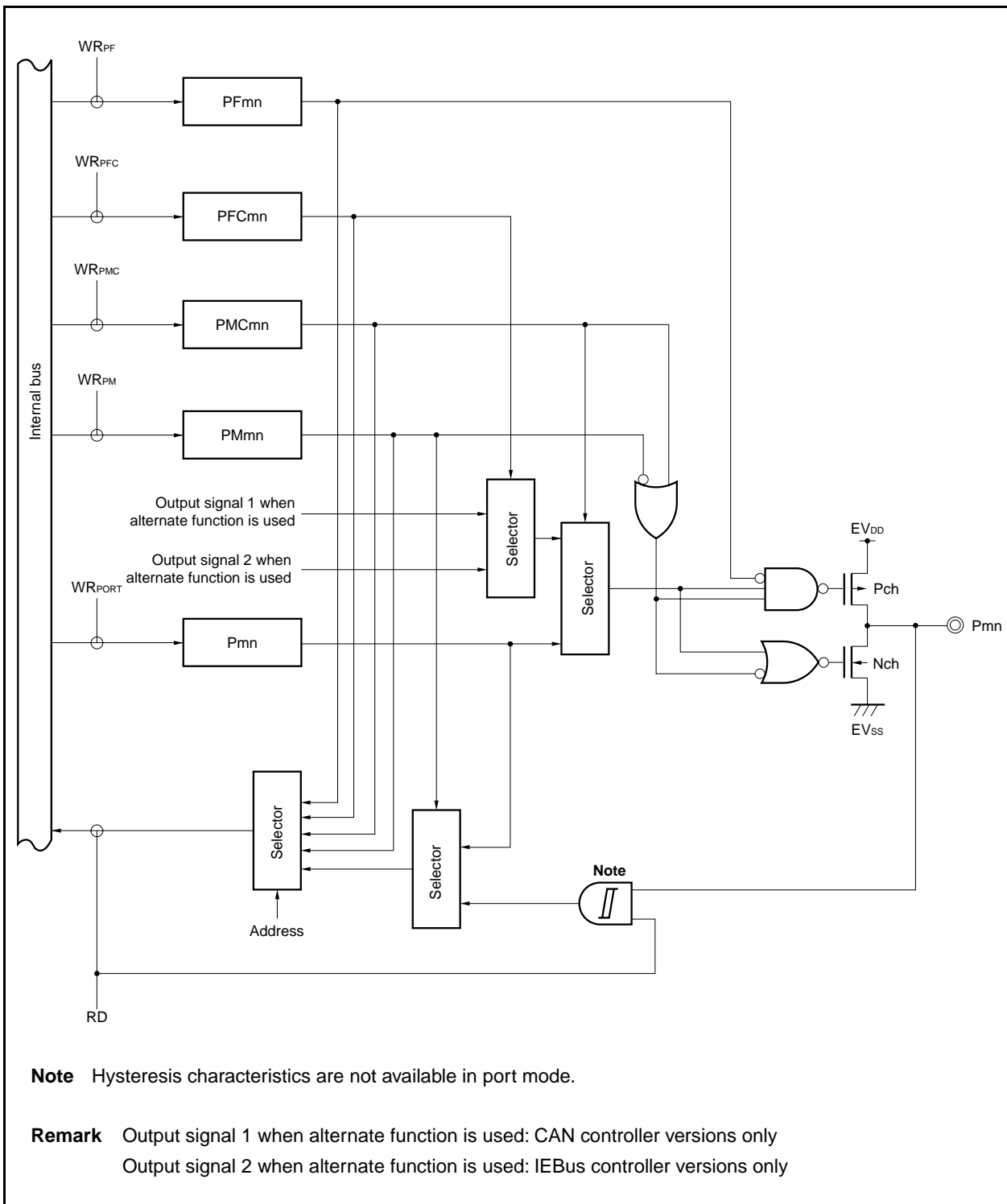
Figure 4-15. Block Diagram of Type G-3
