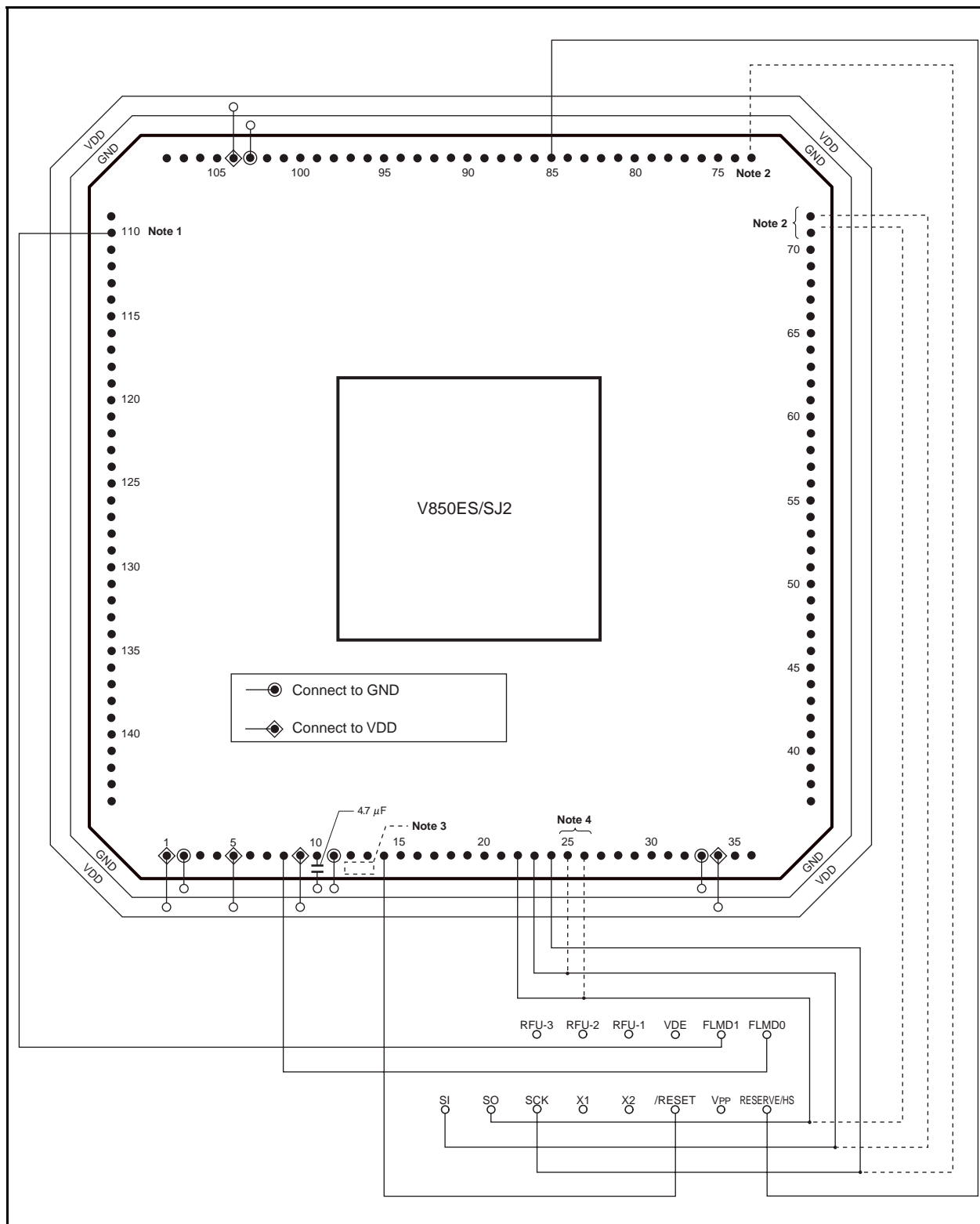
★ Figure 30-6. Example of Wiring of V850ES/SJ2 Flash Writing Adapter (FA-144GJ-UEN) (In CSIB0 + HS Mode) (1/2)
