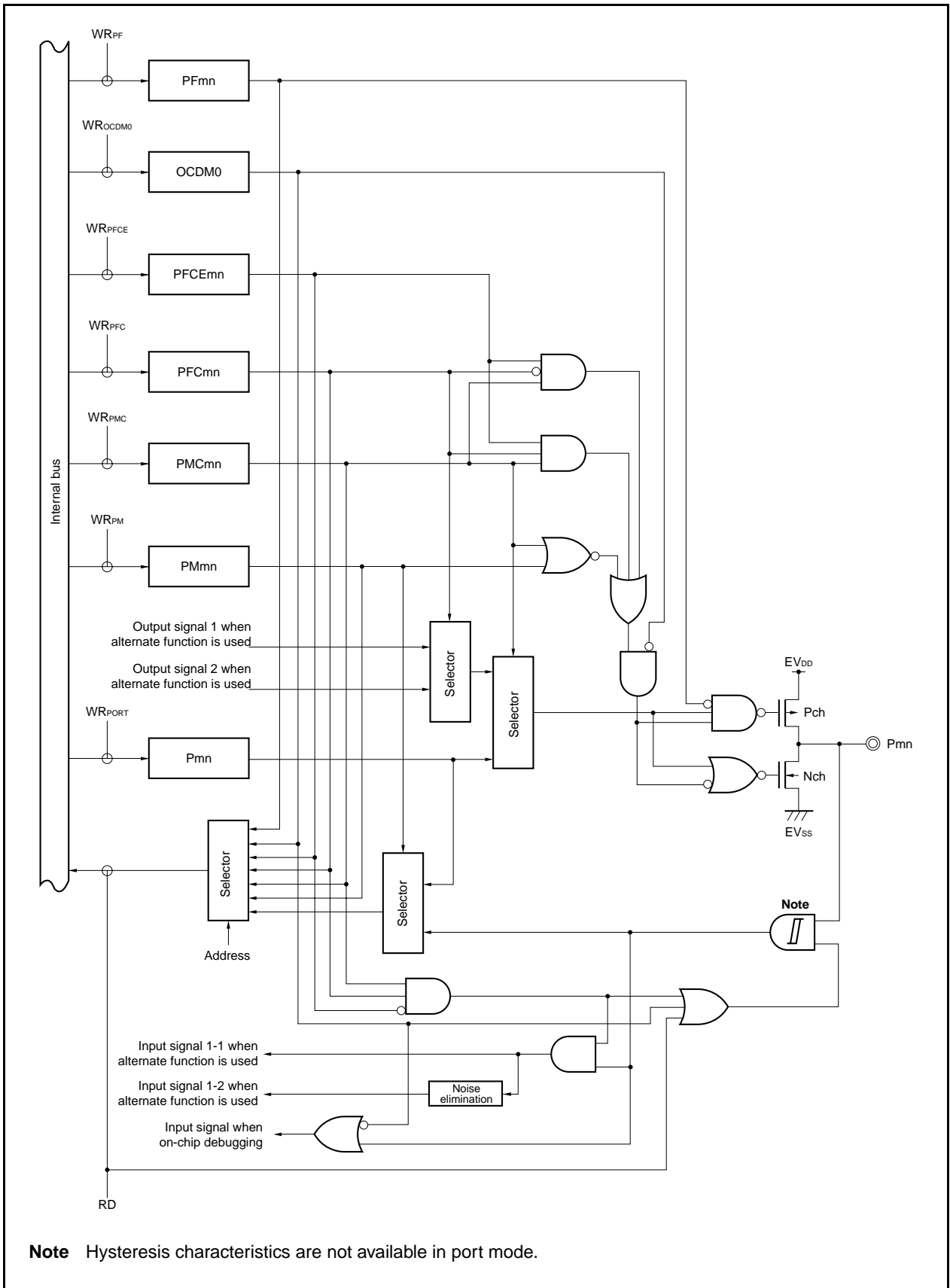
Figure 4-29. Block Diagram of Type U-6
