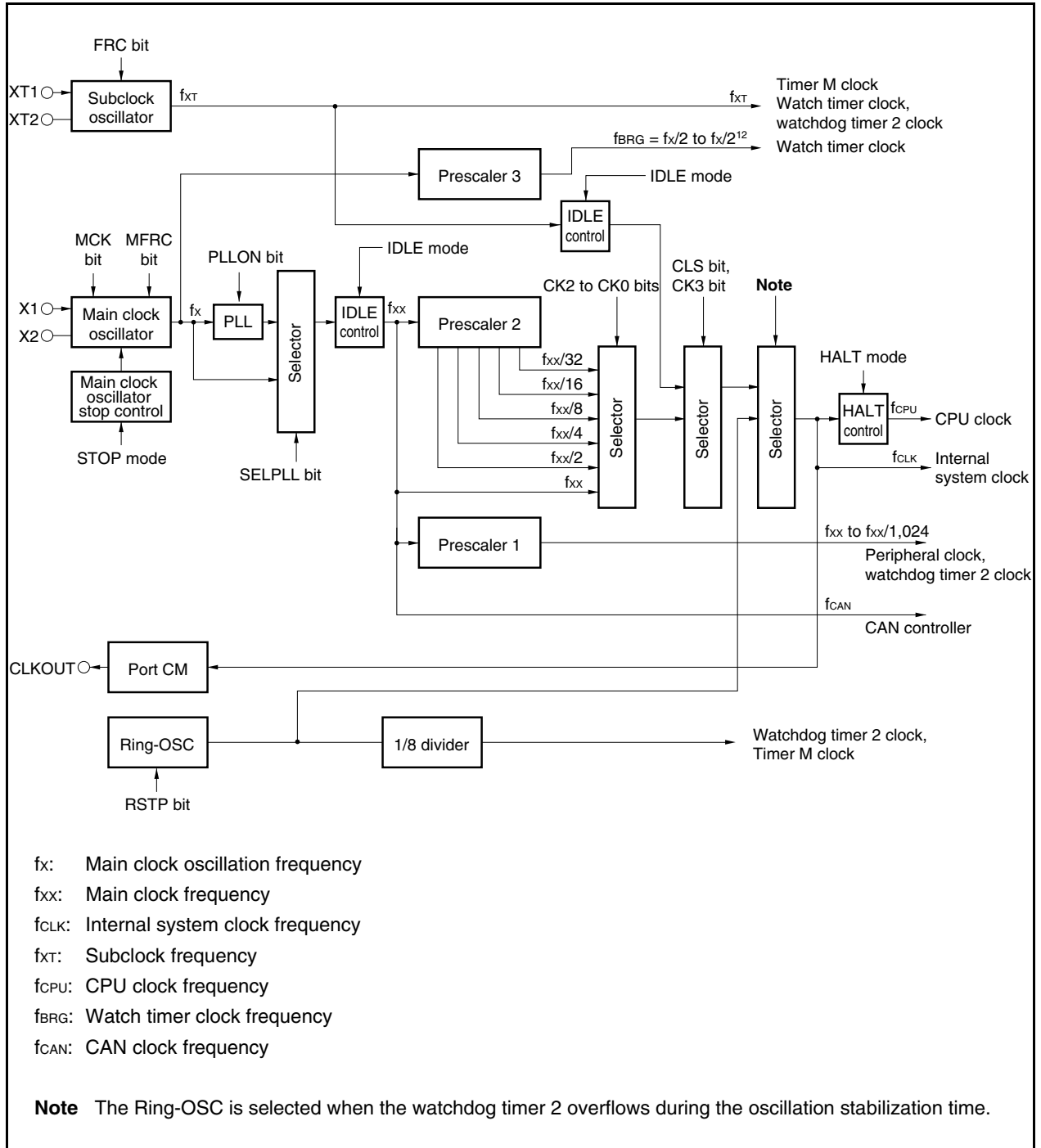
Figure 6-1. Clock Generator
