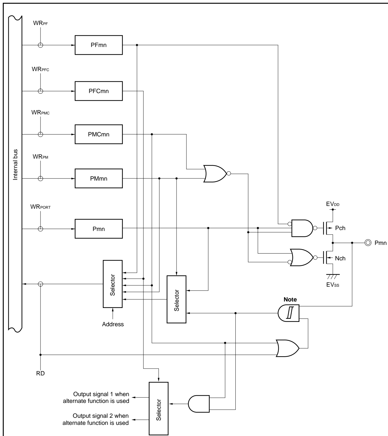
Figure 4-16. Block Diagram of Type G-4
