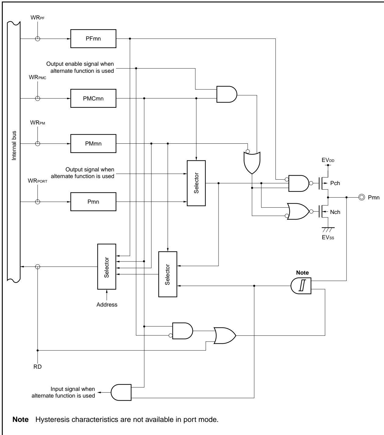
Figure 4-12. Block Diagram of Type E-3
