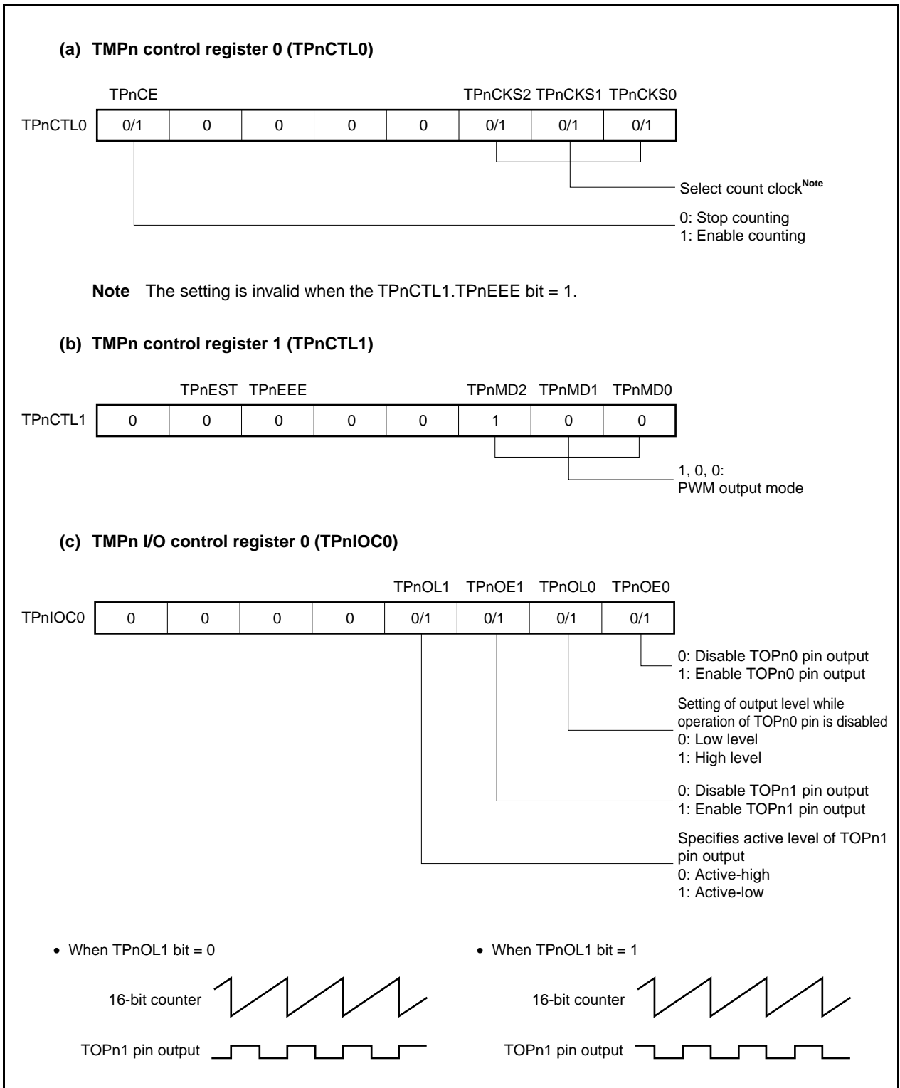
Figure 7-26. Setting of Registers in PWM Output Mode (1/2)
