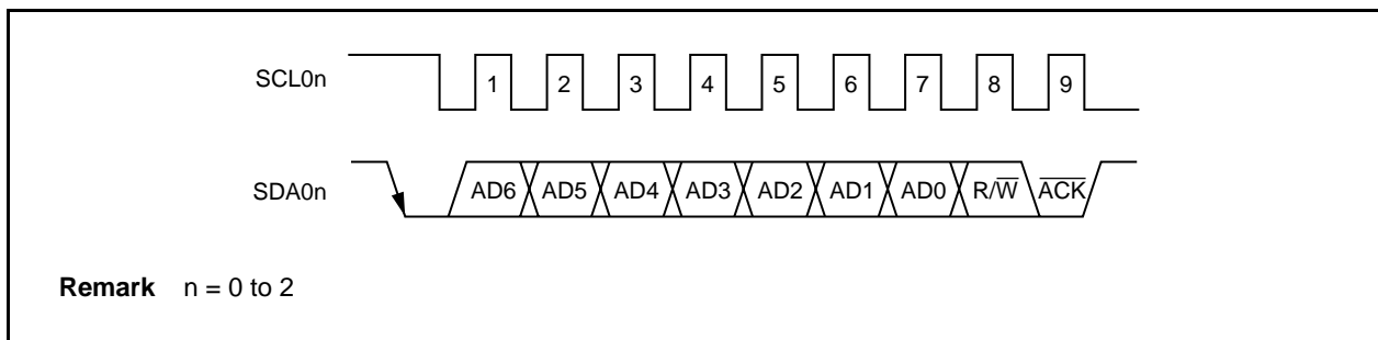
Figure 17-11. \overline{\text{ACK}} Signal
