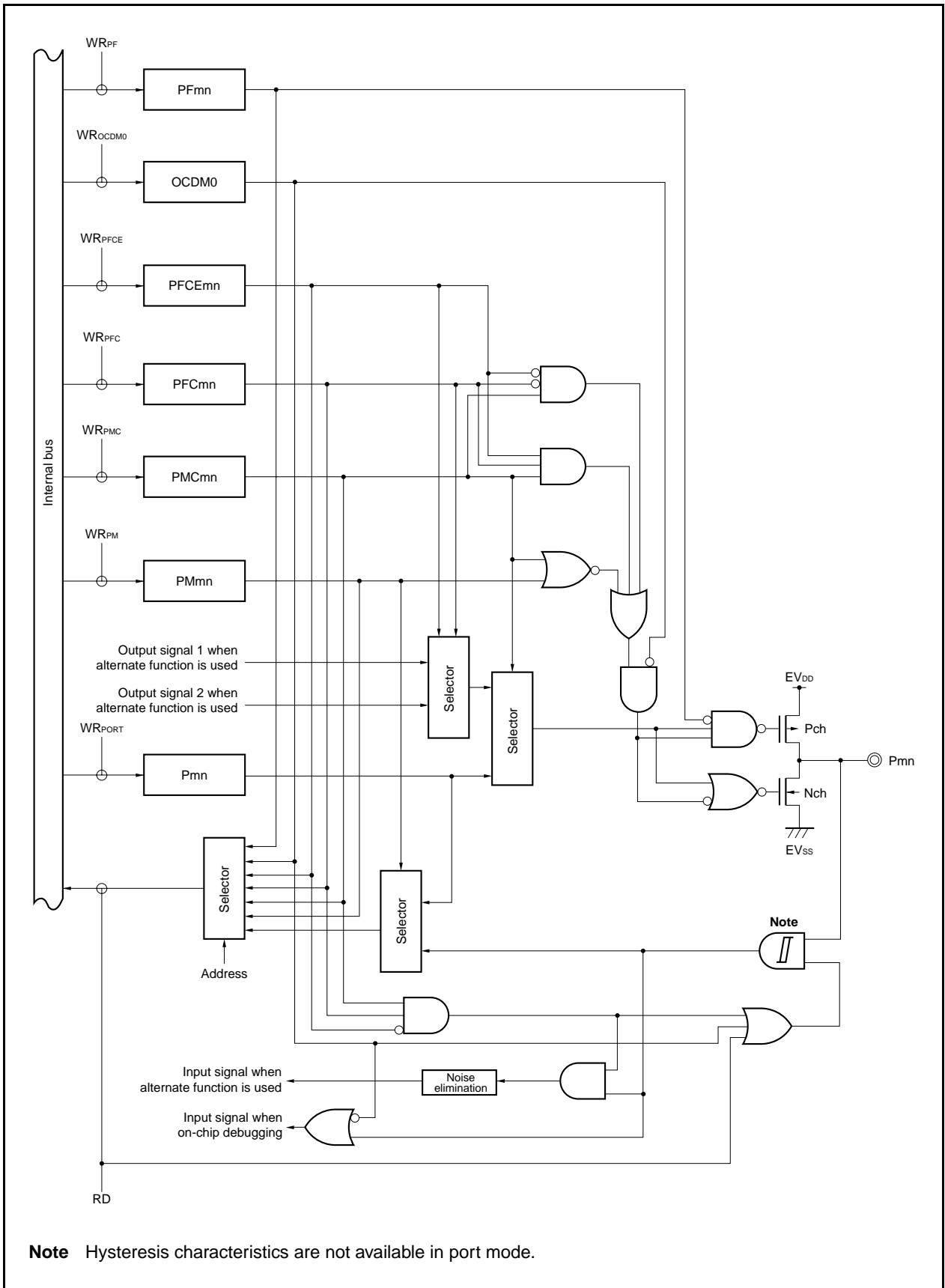
Figure 4-31. Block Diagram of Type U-8
