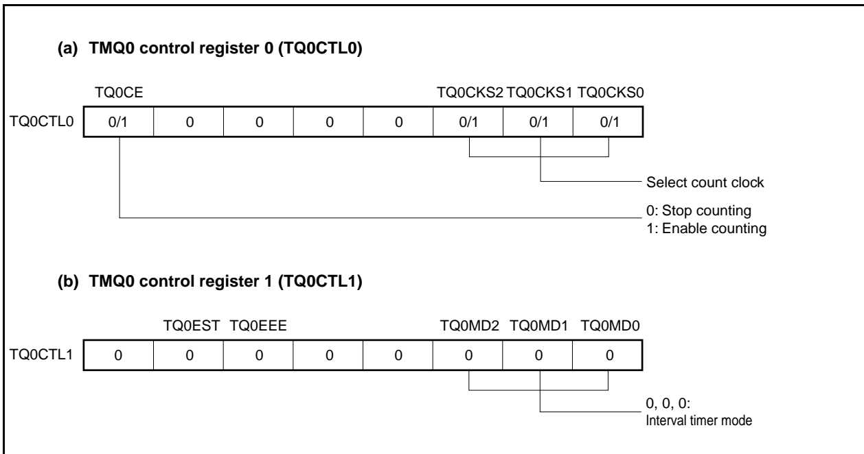
Figure 8-4. Register Setting for Interval Timer Mode Operation (1/2)
