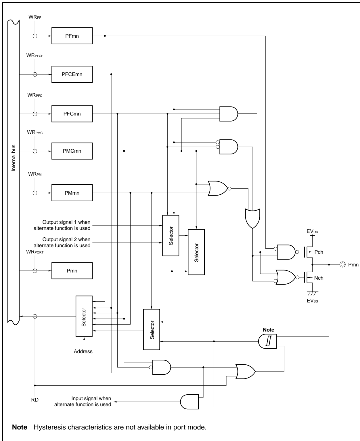
Figure 4-36. Block Diagram of Type U-13
