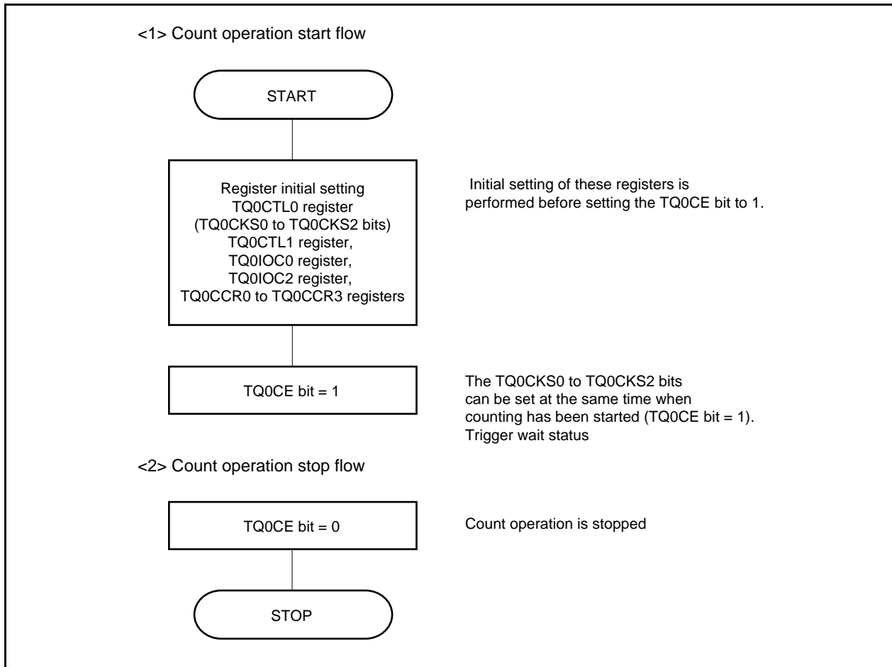
Figure 8-23. Software Processing Flow in One-Shot Pulse Output Mode (2/2)
