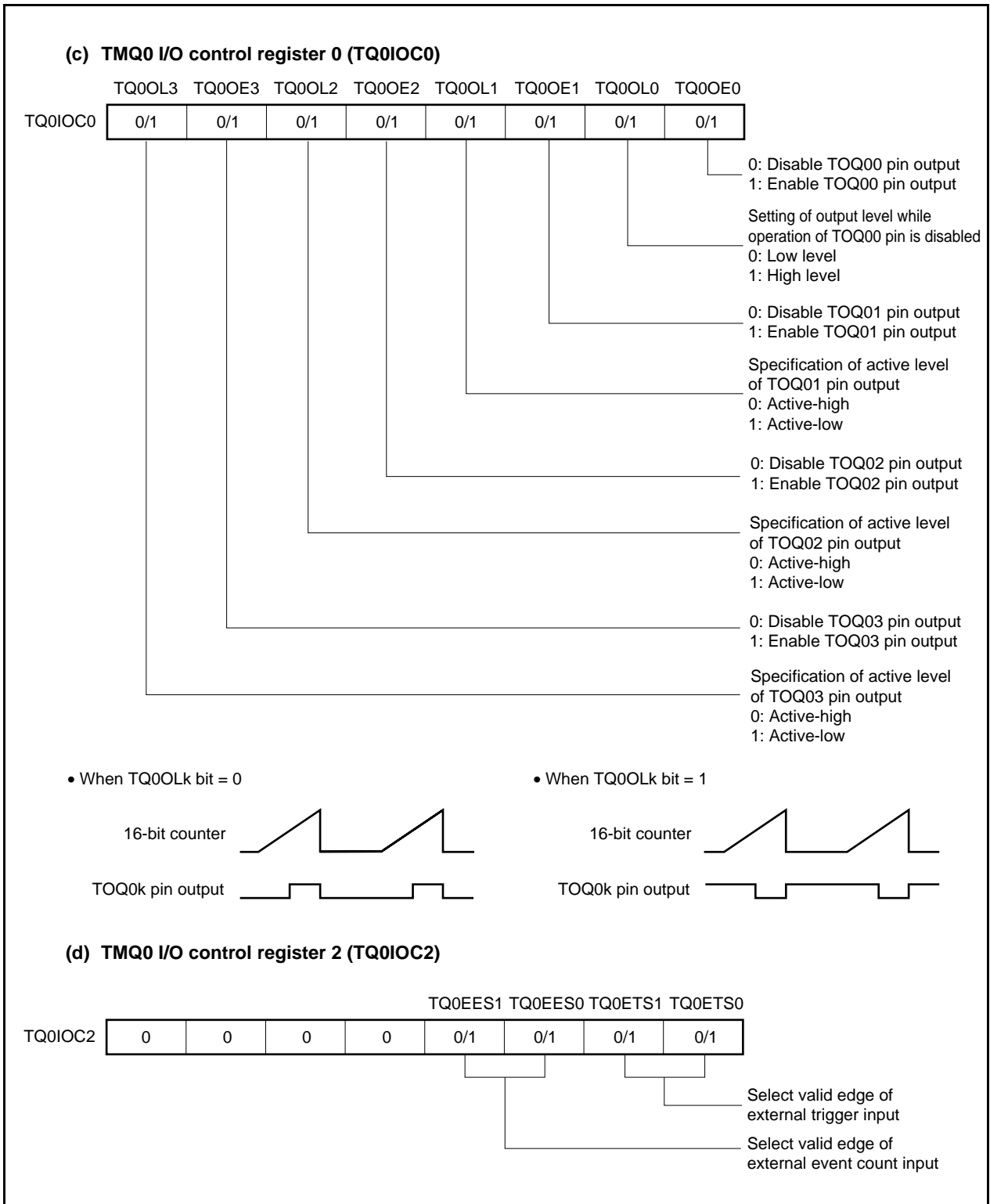
Figure 8-22. Register Setting in One-Shot Pulse Output Mode (2/3)
