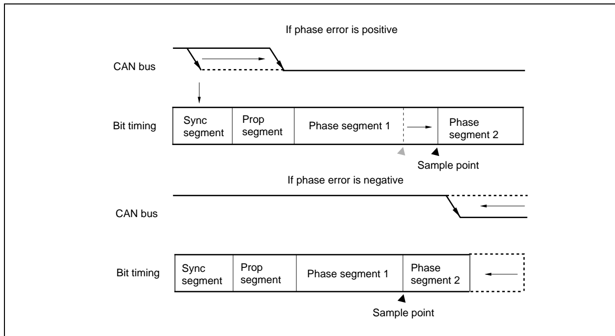
Figure 19-21. Resynchronization
