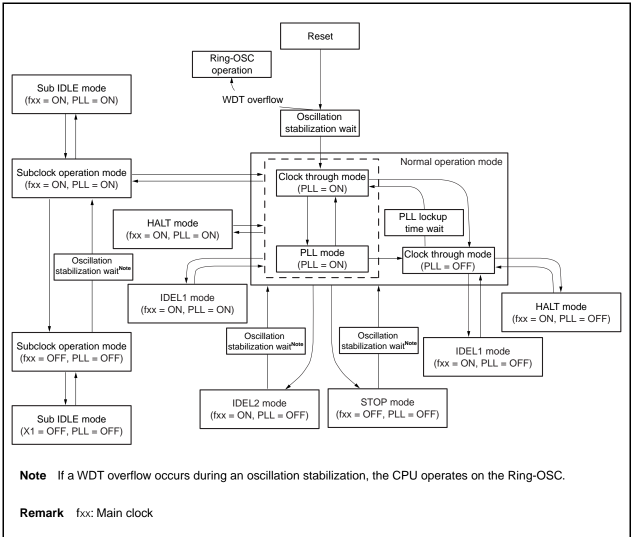
Figure 24-1. Status Transition
