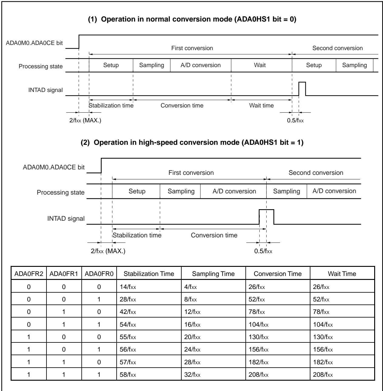
Figure 13-3. Conversion Operation Timing (Continuous Conversion)
