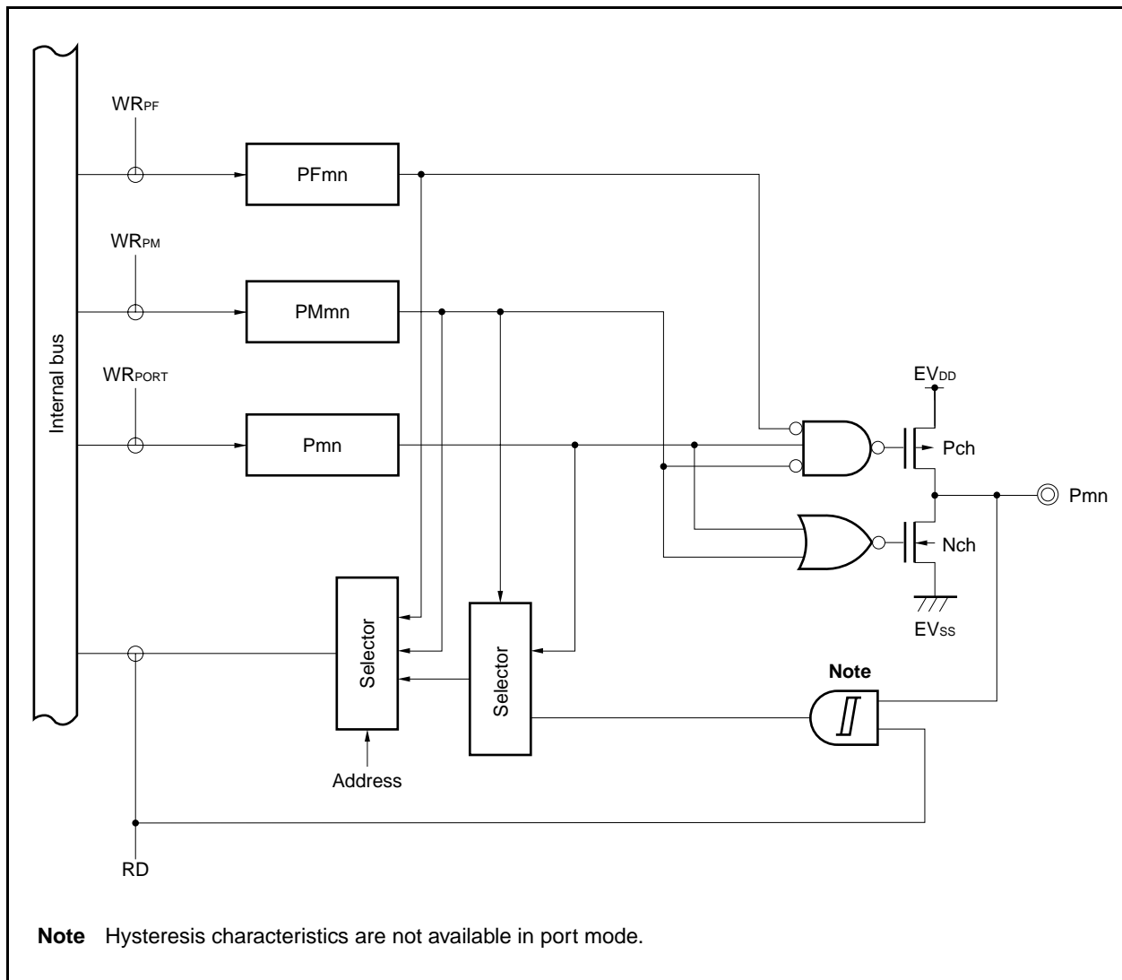
Figure 4-6. Block Diagram of Type C-1
