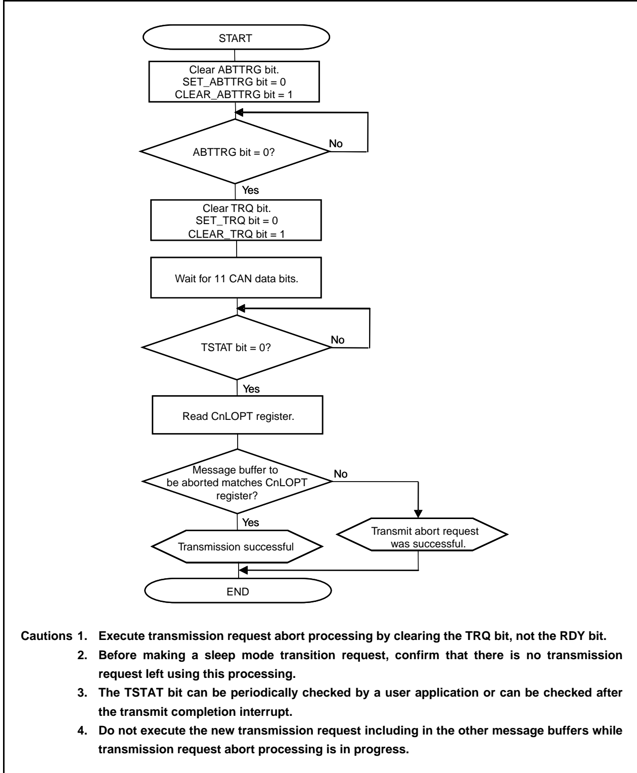
Figure 19-46. Transmission Abort Processing Except for ABT Transmission (Normal Operation Mode with ABT)
