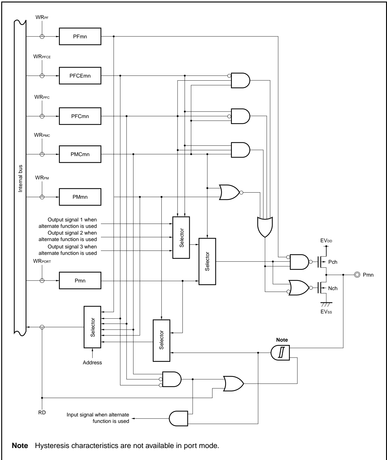
Figure 4-25. Block Diagram of Type U-2
