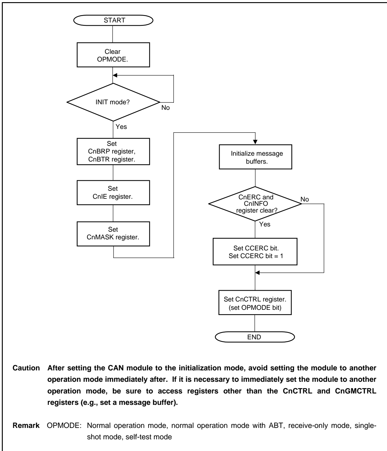
Figure 19-36. Re-initialization
