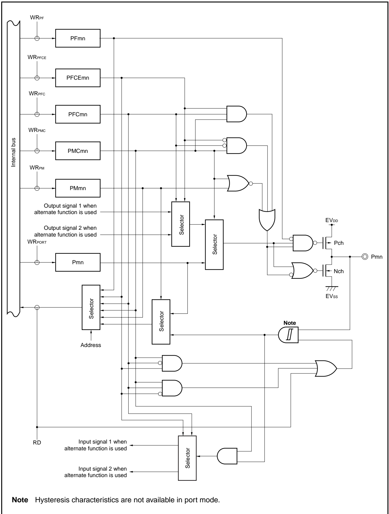
Figure 4-37. Block Diagram of Type U-14
