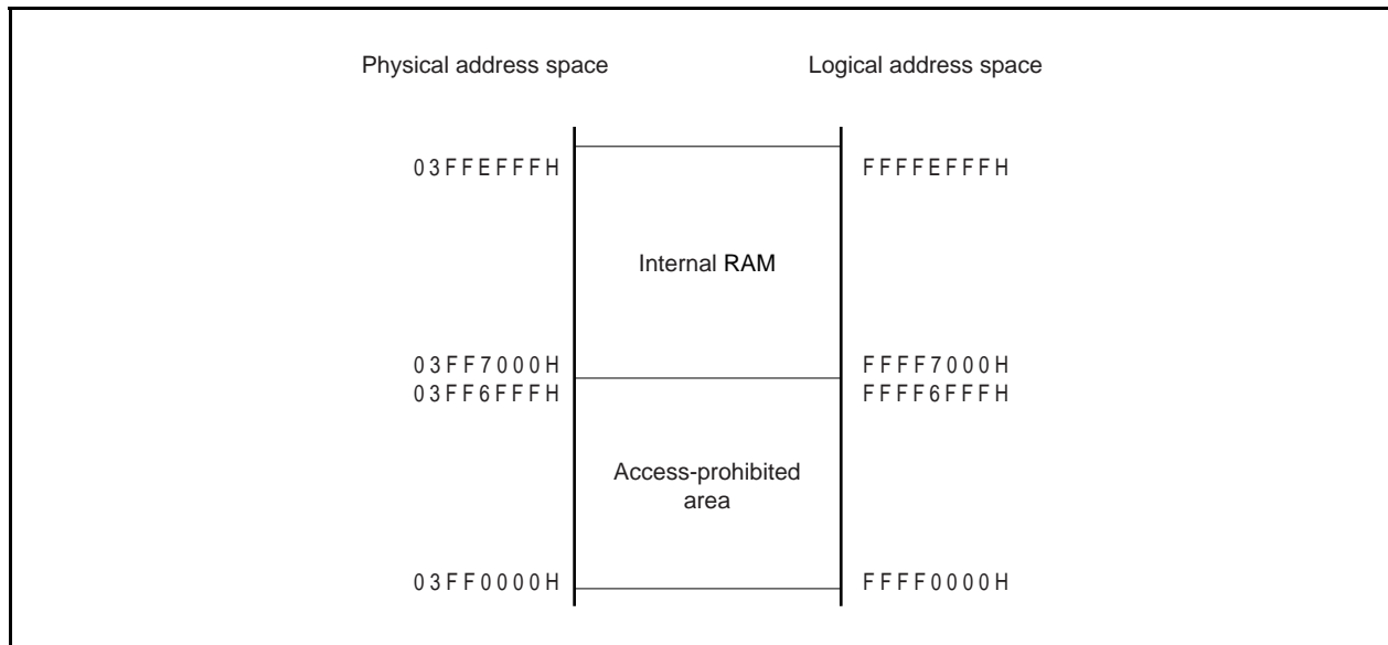
Figure 3-7. Internal RAM Area (32 KB)
