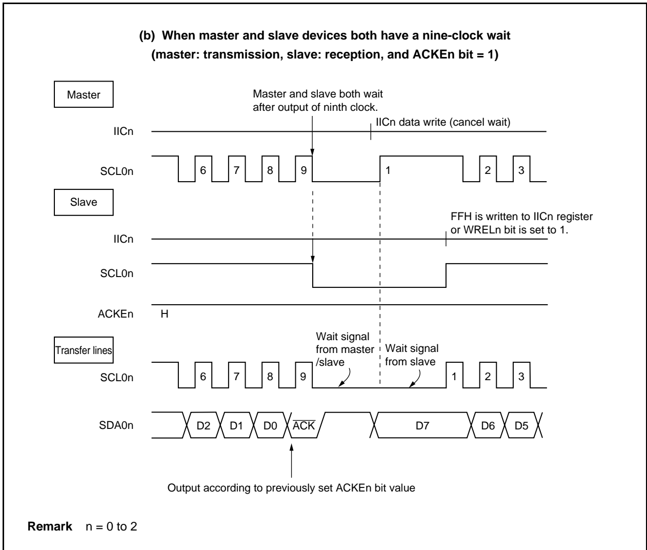
Figure 17-13. Wait Signal (2/2)
