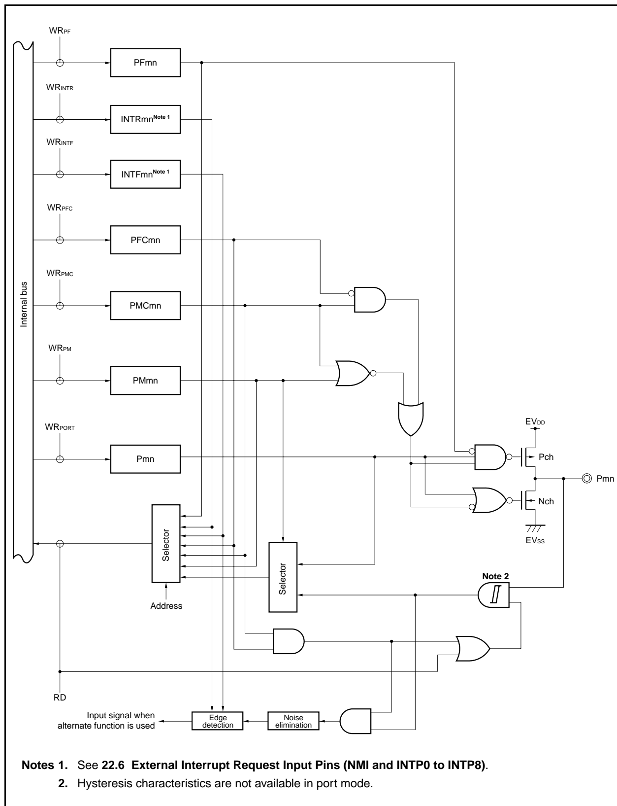
Figure 4-22. Block Diagram of Type N-2
