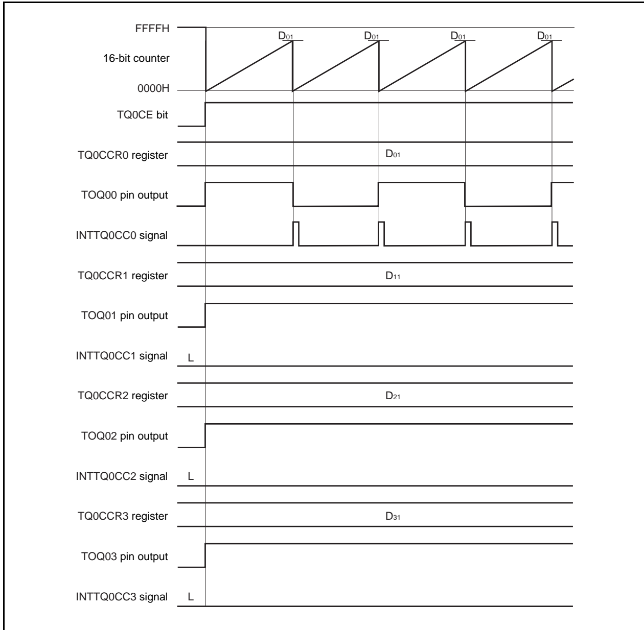
Figure 8-15. Timing Chart When D_{01} < D_{k1}
