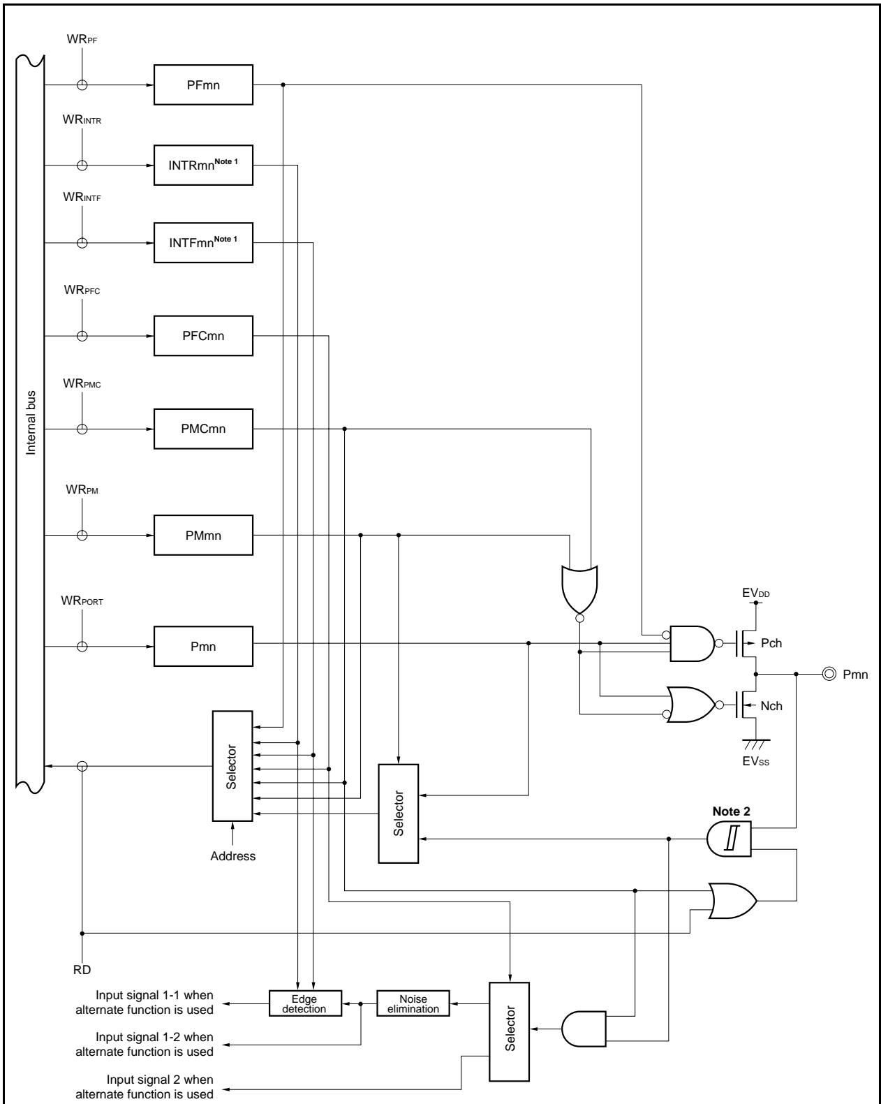
Figure 4-23. Block Diagram of Type N-3
