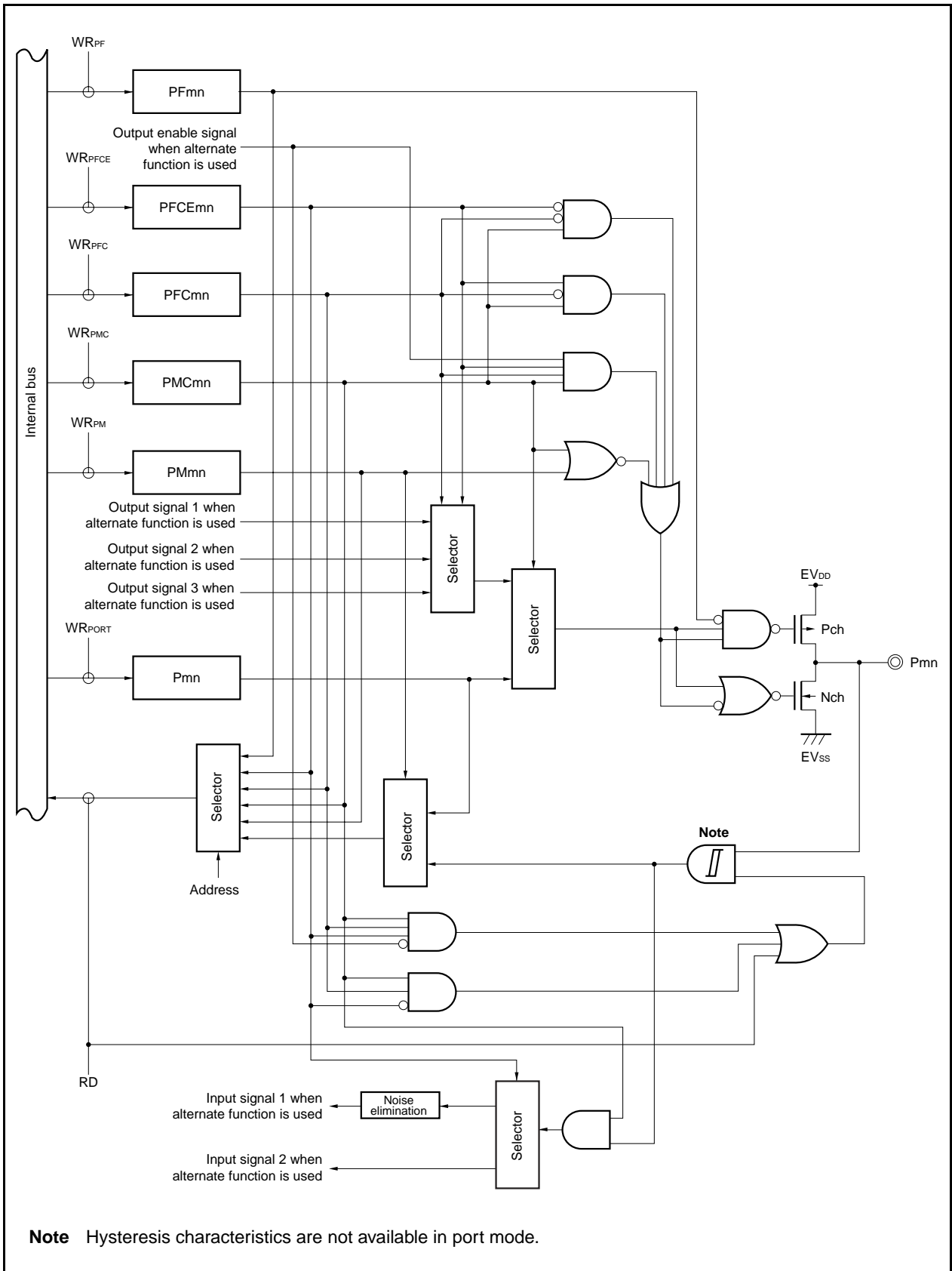
Figure 4-33. Block Diagram of Type U-10
