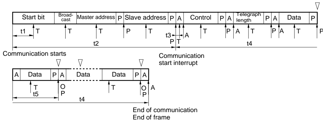
Figure 18-33. Slave Reception (Interval of Interrupt Request Signal Occurrence)
