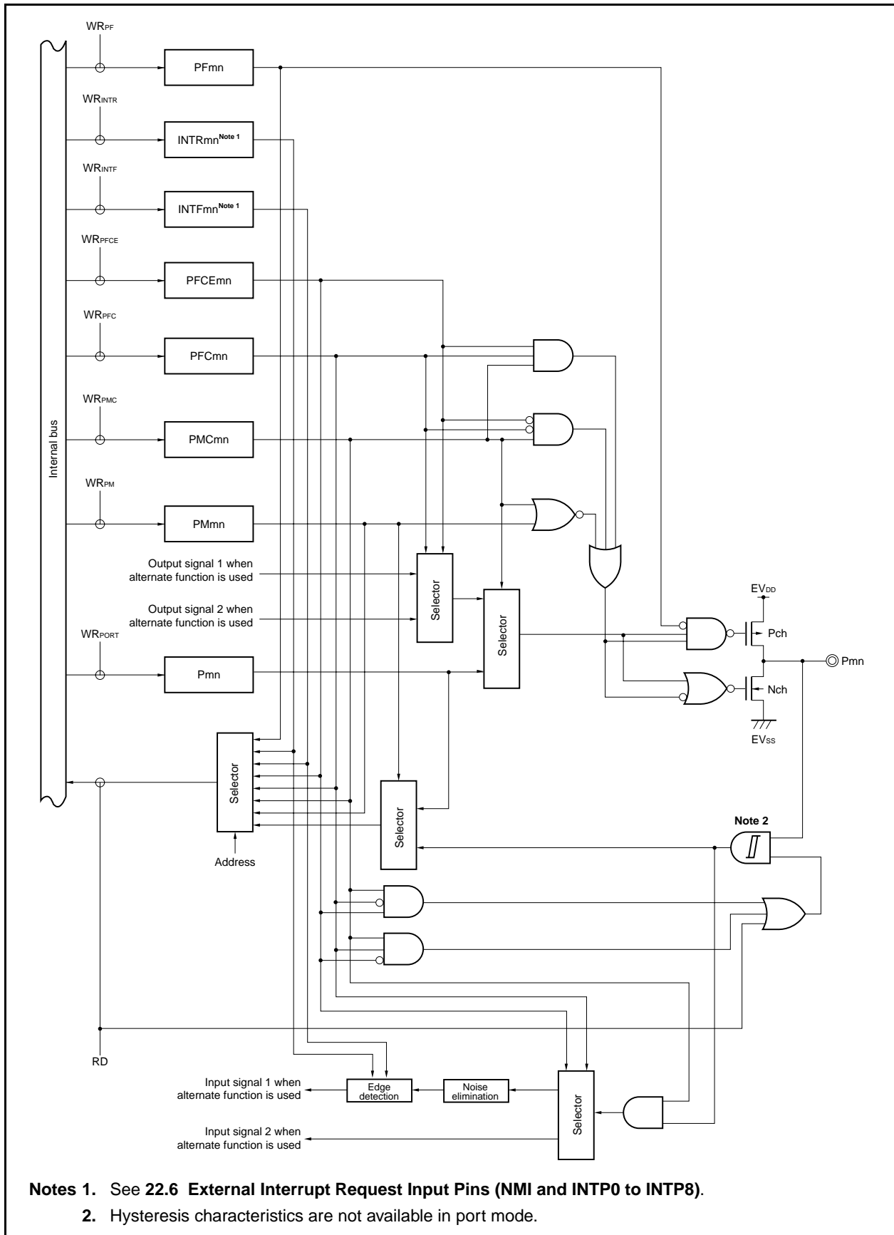
Figure 4-38. Block Diagram of Type U-15
