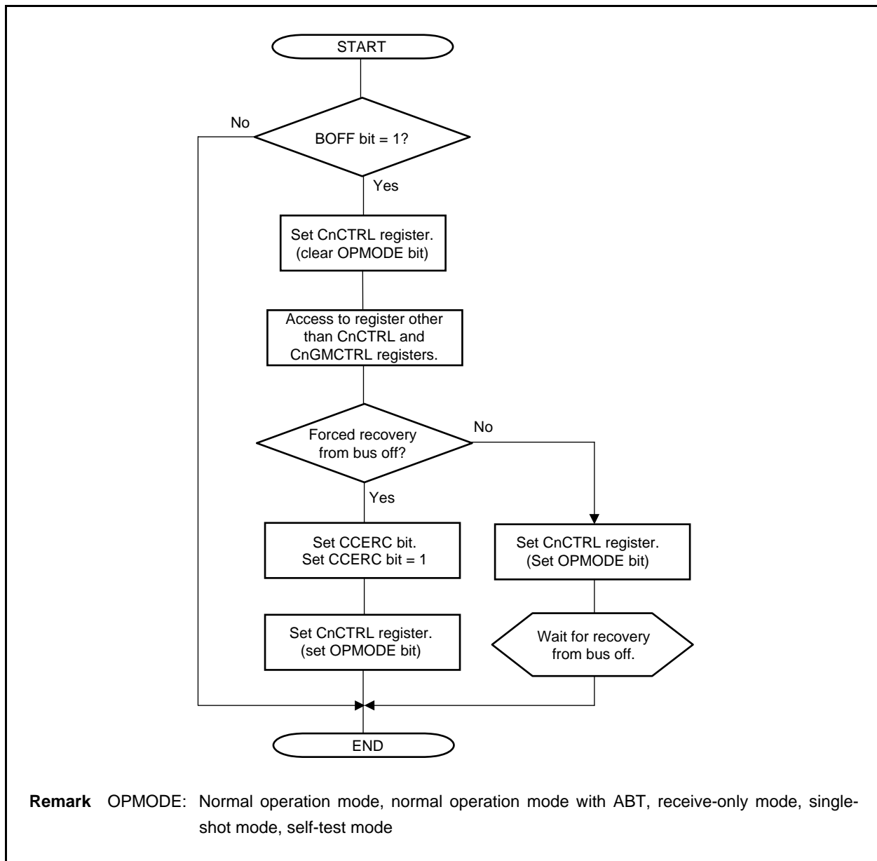
Figure 19-53. Bus-off Recovery
