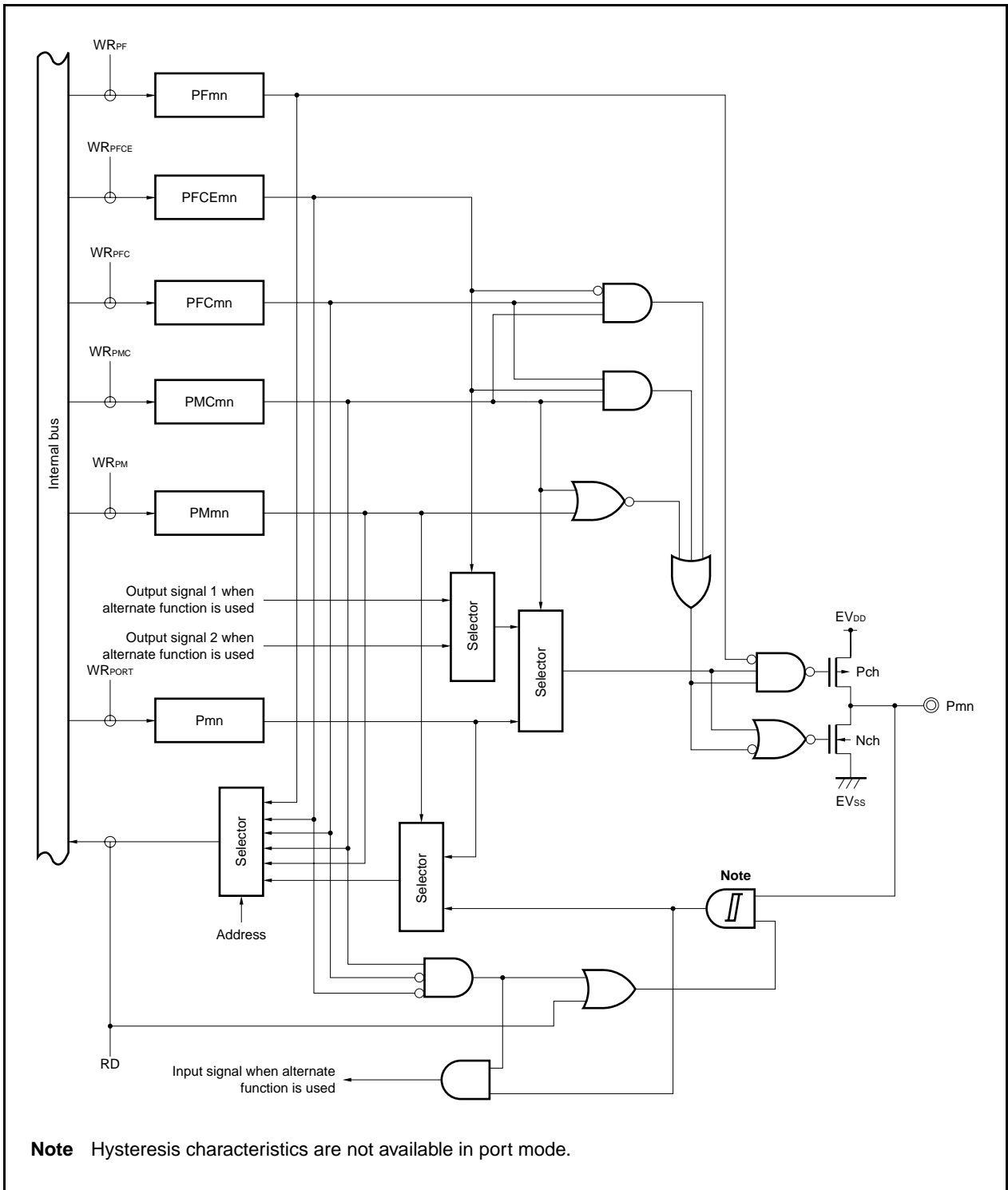
Figure 4-27. Block Diagram of Type U-4
