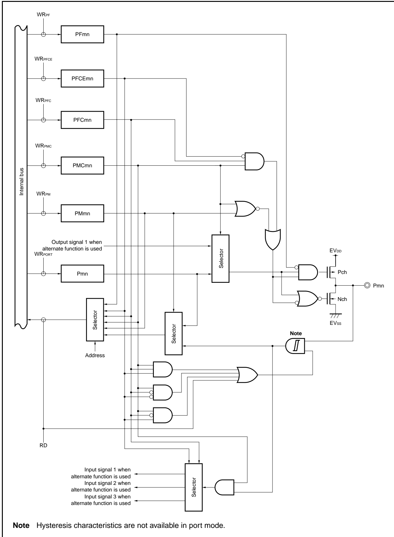
Figure 4-26. Block Diagram of Type U-3
