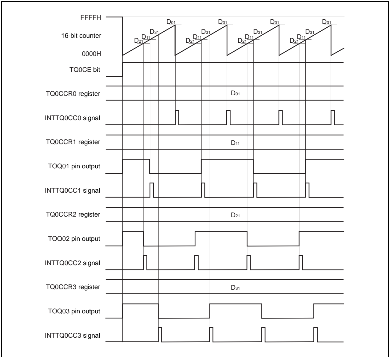
Figure 8-14. Timing Chart When D_{01} \geq D_{k1}
