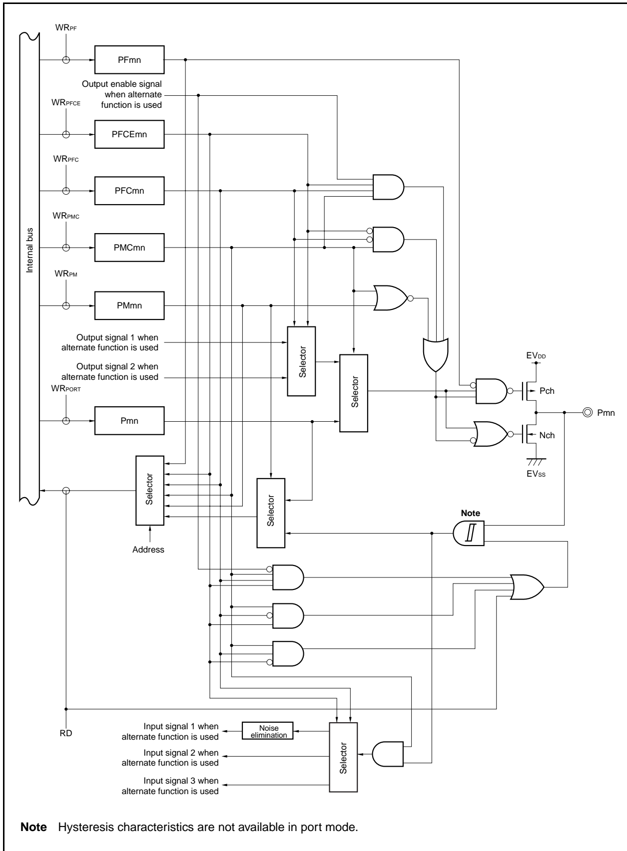
Figure 4-34. Block Diagram of Type U-11
