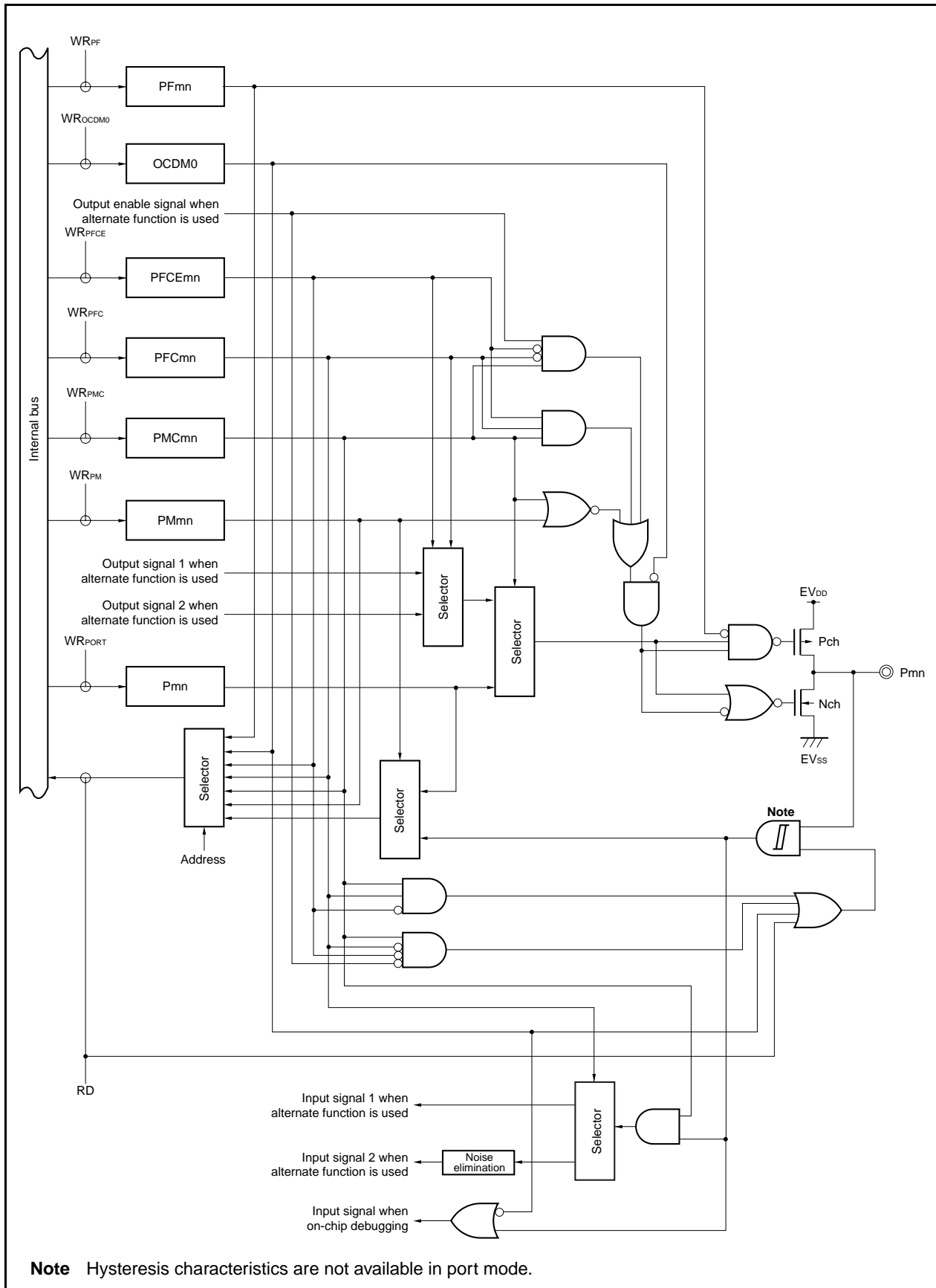
Figure 4-32. Block Diagram of Type U-9
